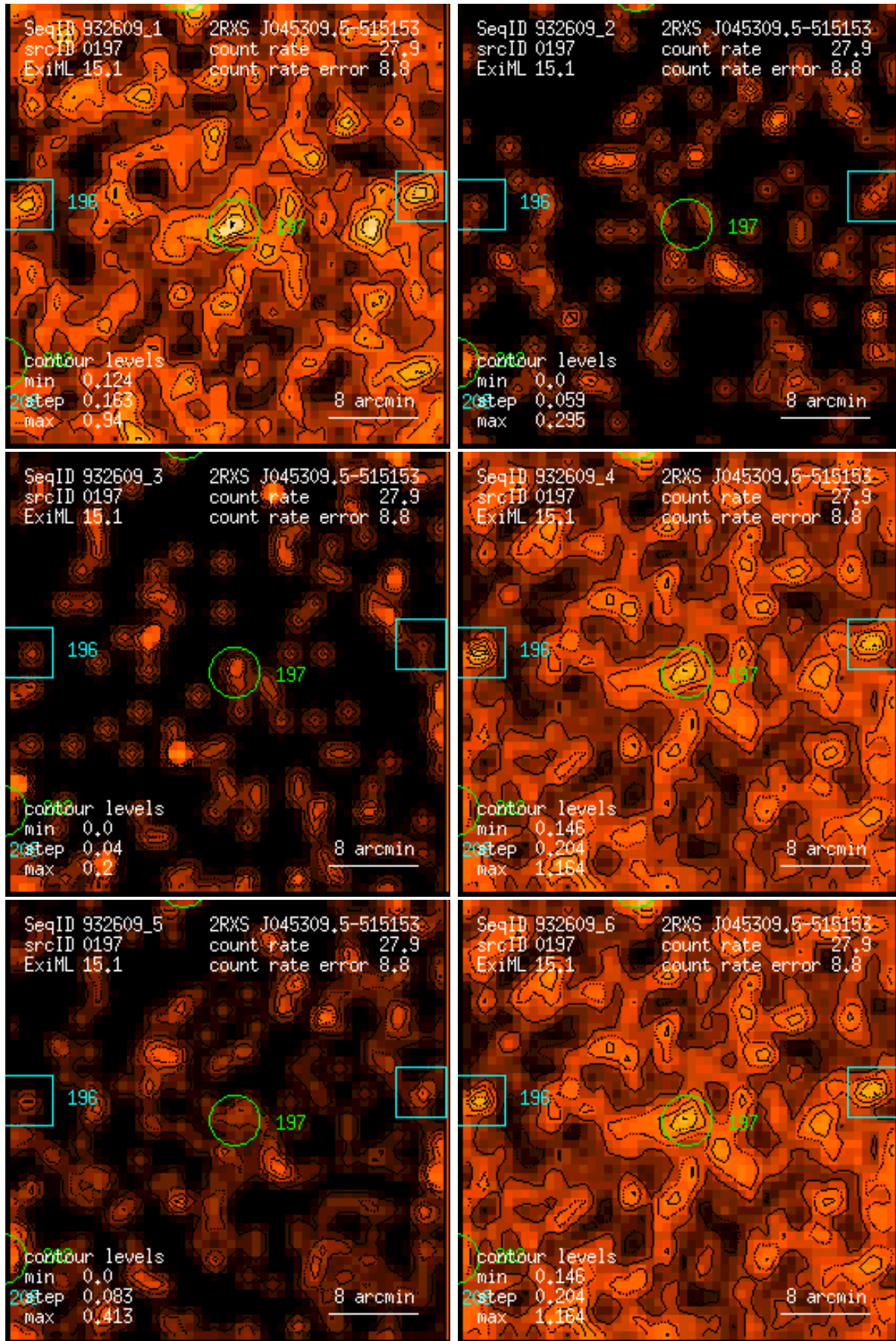
Figure 197: RASS 932609: detection 0197: band rate images, Gaussian filter: (1) PSPC channels 11 – 41, (2) 52 – 90, (3) 91 – 201, (4) 11 – 235, (5) 52 – 201, (6) 11 – 201. Broad band rates in counts/ks. Band rate contour levels in counts/ks/arcmin 2 .
