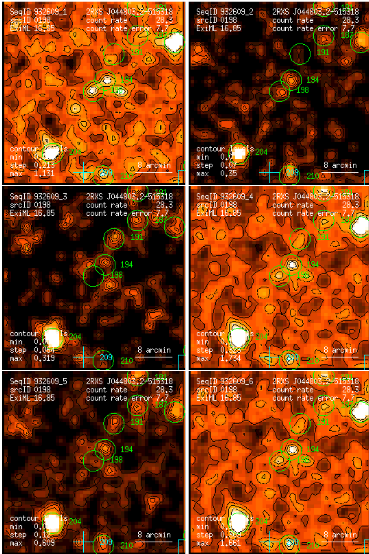
Figure 198: RASS 932609: detection 0198: band rate images, Gaussian filter: (1) PSPC channels 11 – 41, (2) 52 – 90, (3) 91 – 201, (4) 11 – 235, (5) 52 – 201, (6) 11 – 201. Broad band rates in counts/ks. Band rate contour levels in counts/ks/arcmin 2 .
