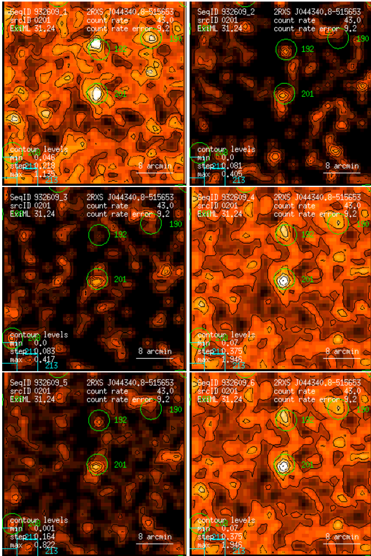
Figure 201: RASS 932609: detection 0201: band rate images, Gaussian filter: (1) PSPC channels 11 – 41, (2) 52 – 90, (3) 91 – 201, (4) 11 – 235, (5) 52 – 201, (6) 11 – 201. Broad band rates in counts/ks. Band rate contour levels in counts/ks/arcmin 2 .
