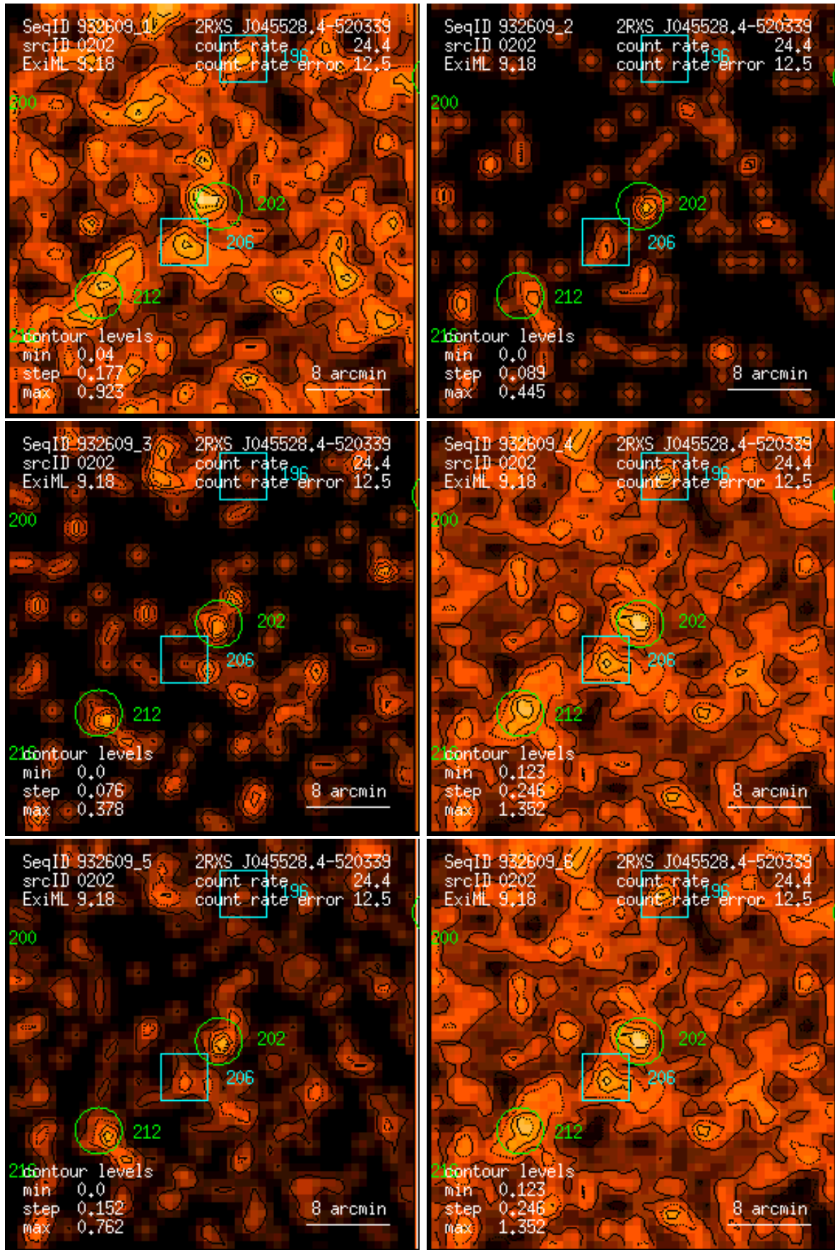
Figure 202: RASS 932609: detection 0202: band rate images, Gaussian filter: (1) PSPC channels 11 – 41, (2) 52 – 90, (3) 91 – 201, (4) 11 – 235, (5) 52 – 201, (6) 11 – 201. Broad band rates in counts/ks. Band rate contour levels in counts/ks/arcmin 2 .
