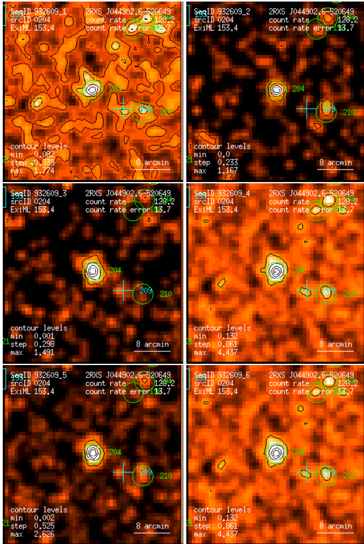
Figure 204: RASS 932609: detection 0204: band rate images, Gaussian filter: (1) PSPC channels 11 – 41, (2) 52 – 90, (3) 91 – 201, (4) 11 – 235, (5) 52 – 201, (6) 11 – 201. Broad band rates in counts/ks. Band rate contour levels in counts/ks/arcmin 2 .
