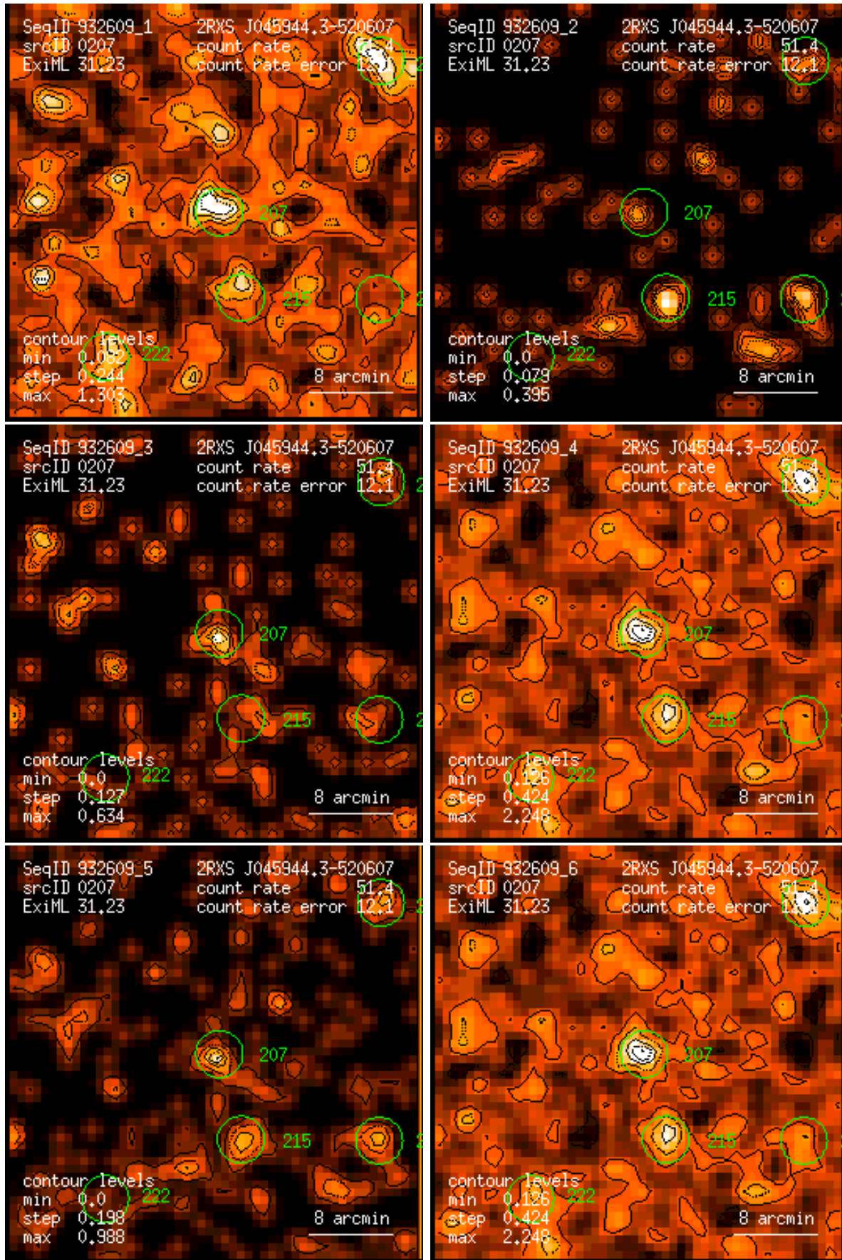
Figure 207: RASS 932609: detection 0207: band rate images, Gaussian filter: (1) PSPC channels 11 – 41, (2) 52 – 90, (3) 91 – 201, (4) 11 – 235, (5) 52 – 201, (6) 11 – 201. Broad band rates in counts/ks. Band rate contour levels in counts/ks/arcmin 2 .
