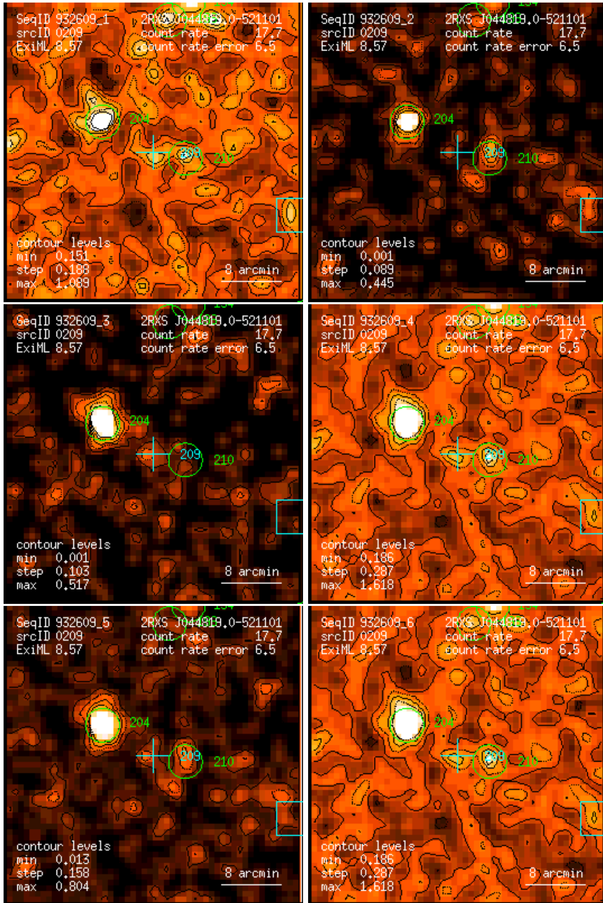
Figure 209: RASS 932609: detection 0209: band rate images, Gaussian filter: (1) PSPC channels 11 – 41, (2) 52 – 90, (3) 91 – 201, (4) 11 – 235, (5) 52 – 201, (6) 11 – 201. Broad band rates in counts/ks. Band rate contour levels in counts/ks/arcmin 2 .
