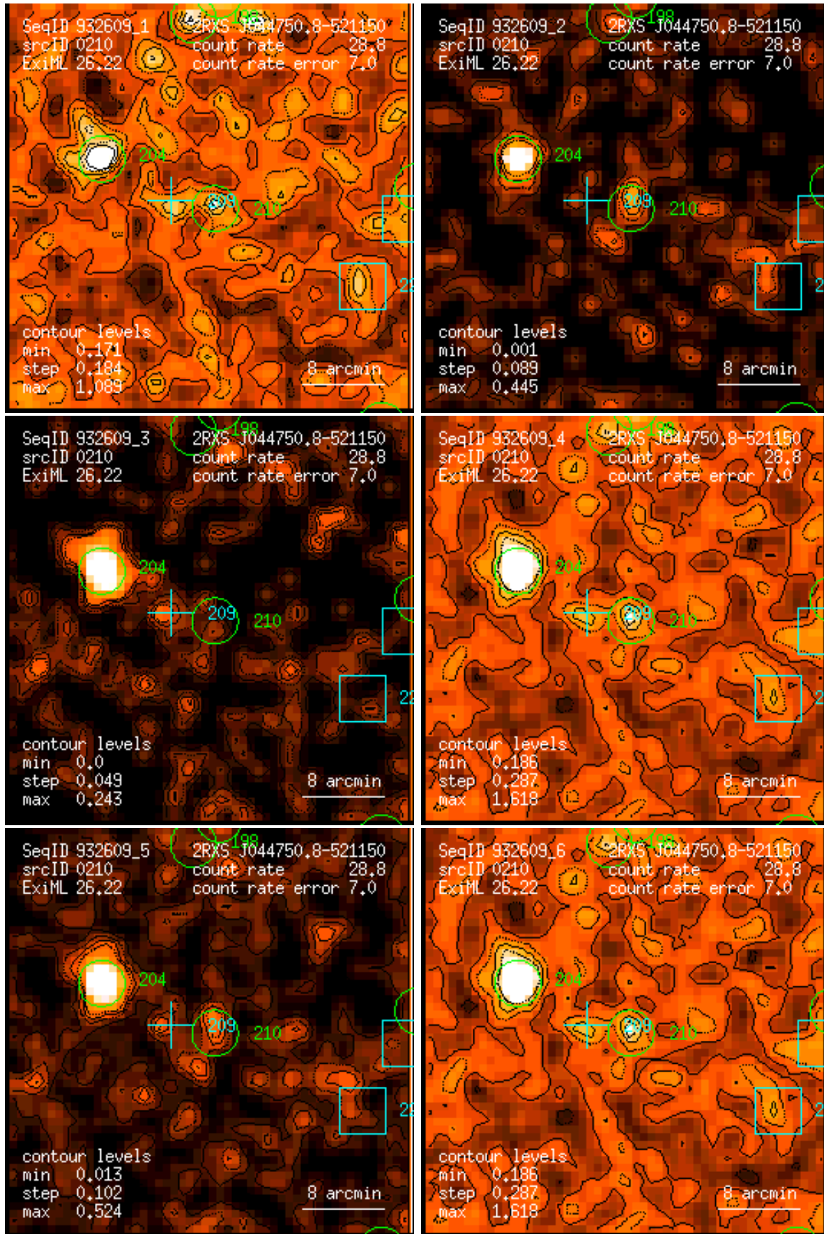
Figure 210: RASS 932609: detection 0210: band rate images, Gaussian filter: (1) PSPC channels 11 – 41, (2) 52 – 90, (3) 91 – 201, (4) 11 – 235, (5) 52 – 201, (6) 11 – 201. Broad band rates in counts/ks. Band rate contour levels in counts/ks/arcmin 2 .
