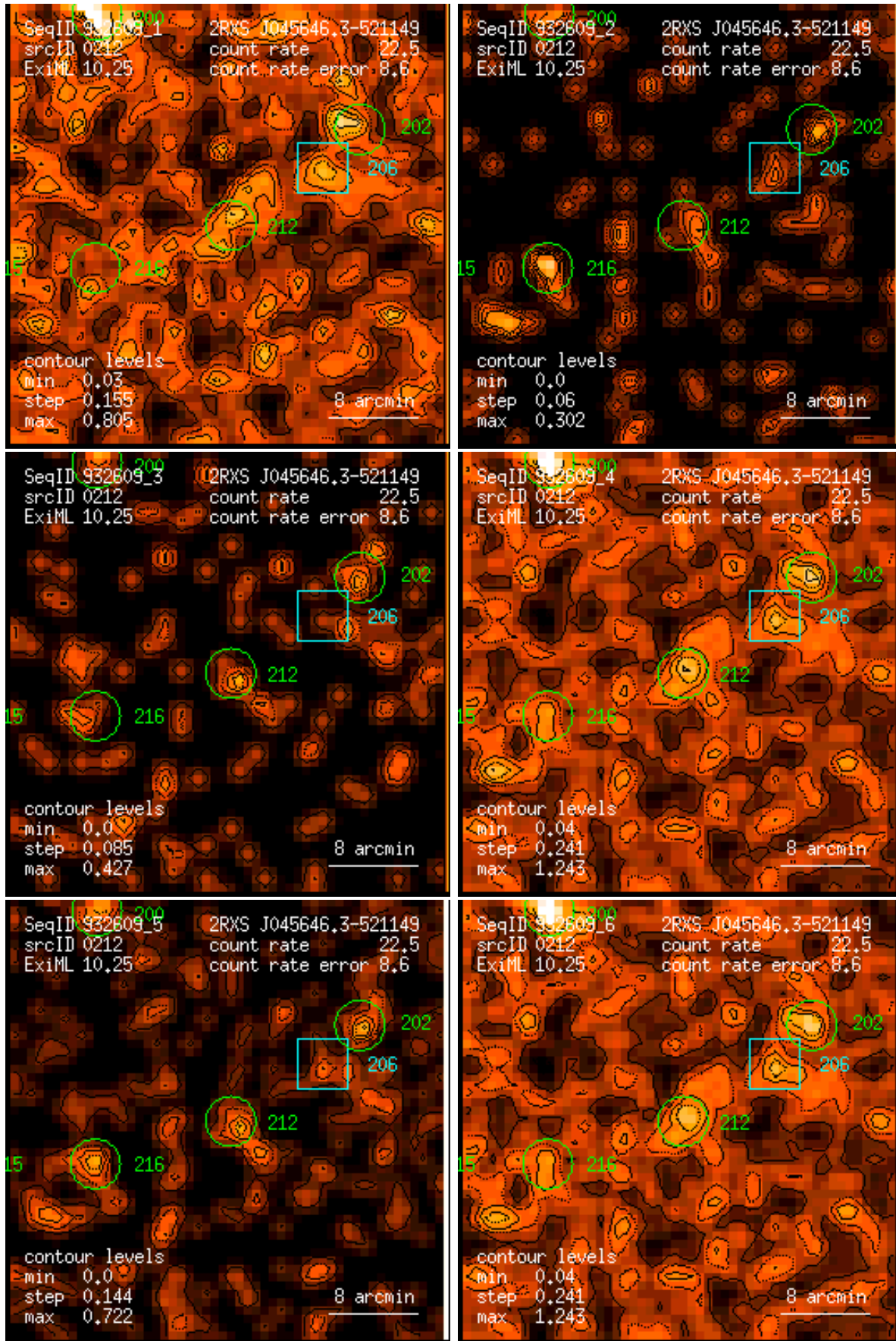
Figure 212: RASS 932609: detection 0212: band rate images, Gaussian filter: (1) PSPC channels 11 – 41, (2) 52 – 90, (3) 91 – 201, (4) 11 – 235, (5) 52 – 201, (6) 11 – 201. Broad band rates in counts/ks. Band rate contour levels in counts/ks/arcmin 2 .
