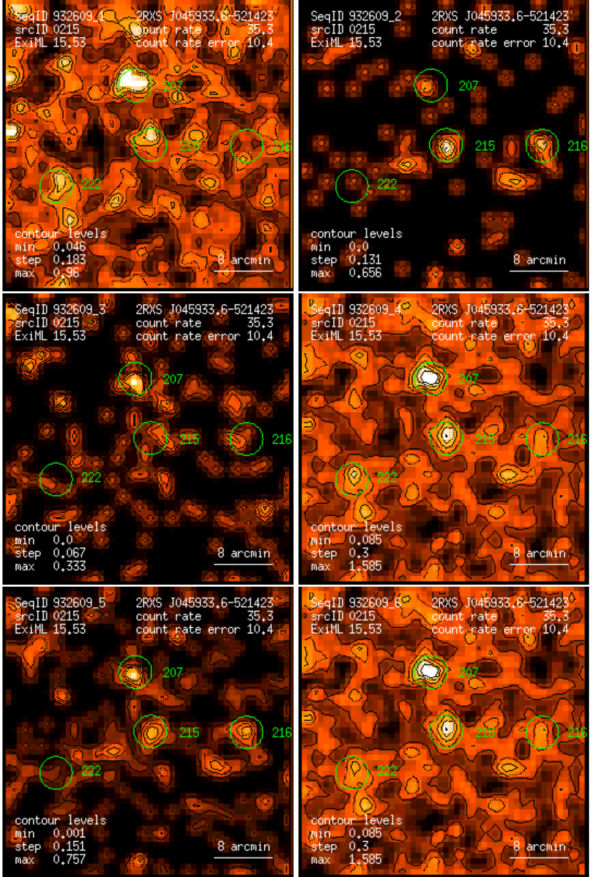
Figure 215: RASS 932609: detection 0215: band rate images, Gaussian filter: (1) PSPC channels 11 – 41, (2) 52 – 90, (3) 91 – 201, (4) 11 – 235, (5) 52 – 201, (6) 11 – 201. Broad band rates in counts/ks. Band rate contour levels in counts/ks/arcmin 2 .
