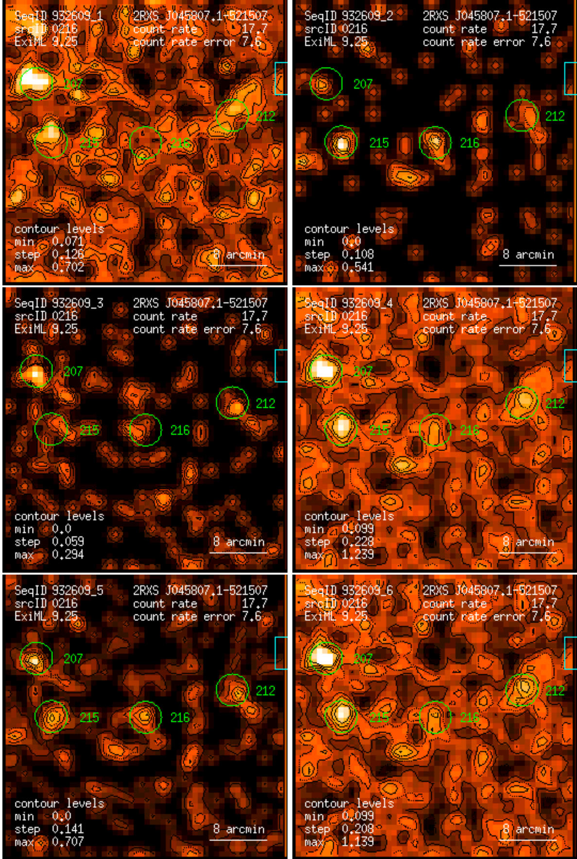
Figure 216: RASS 932609: detection 0216: band rate images, Gaussian filter: (1) PSPC channels 11 – 41, (2) 52 – 90, (3) 91 – 201, (4) 11 – 235, (5) 52 – 201, (6) 11 – 201. Broad band rates in counts/ks. Band rate contour levels in counts/ks/arcmin 2 .
