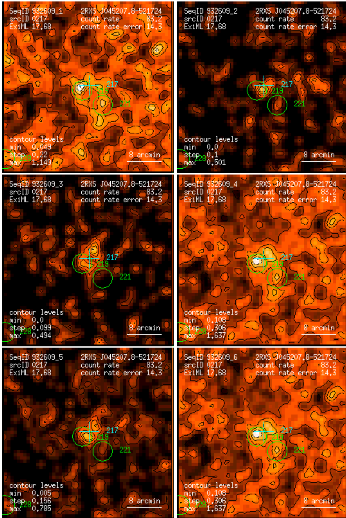
Figure 217: RASS 932609: detection 0217: band rate images, Gaussian filter: (1) PSPC channels 11 – 41, (2) 52 – 90, (3) 91 – 201, (4) 11 – 235, (5) 52 – 201, (6) 11 – 201. Broad band rates in counts/ks. Band rate contour levels in counts/ks/arcmin 2 .
