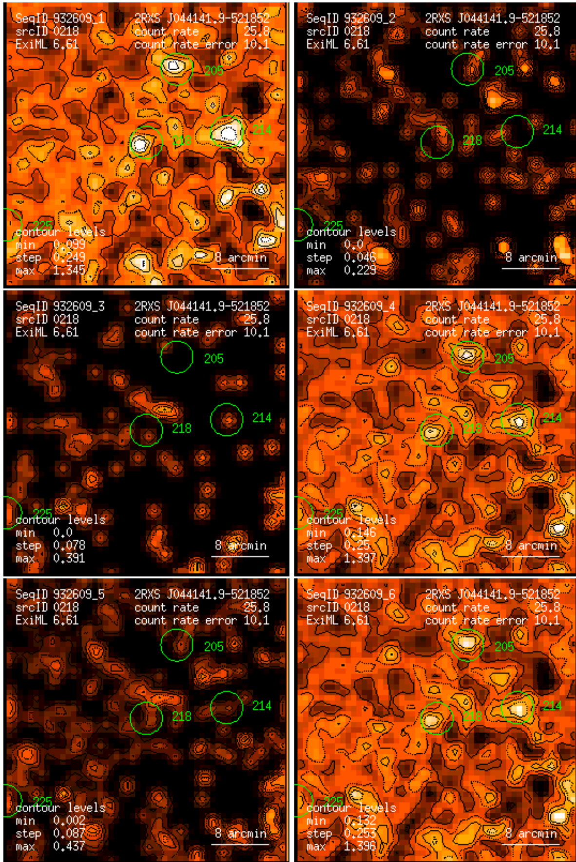
Figure 218: RASS 932609: detection 0218: band rate images, Gaussian filter: (1) PSPC channels 11 – 41, (2) 52 – 90, (3) 91 – 201, (4) 11 – 235, (5) 52 – 201, (6) 11 – 201. Broad band rates in counts/ks. Band rate contour levels in counts/ks/arcmin 2 .
