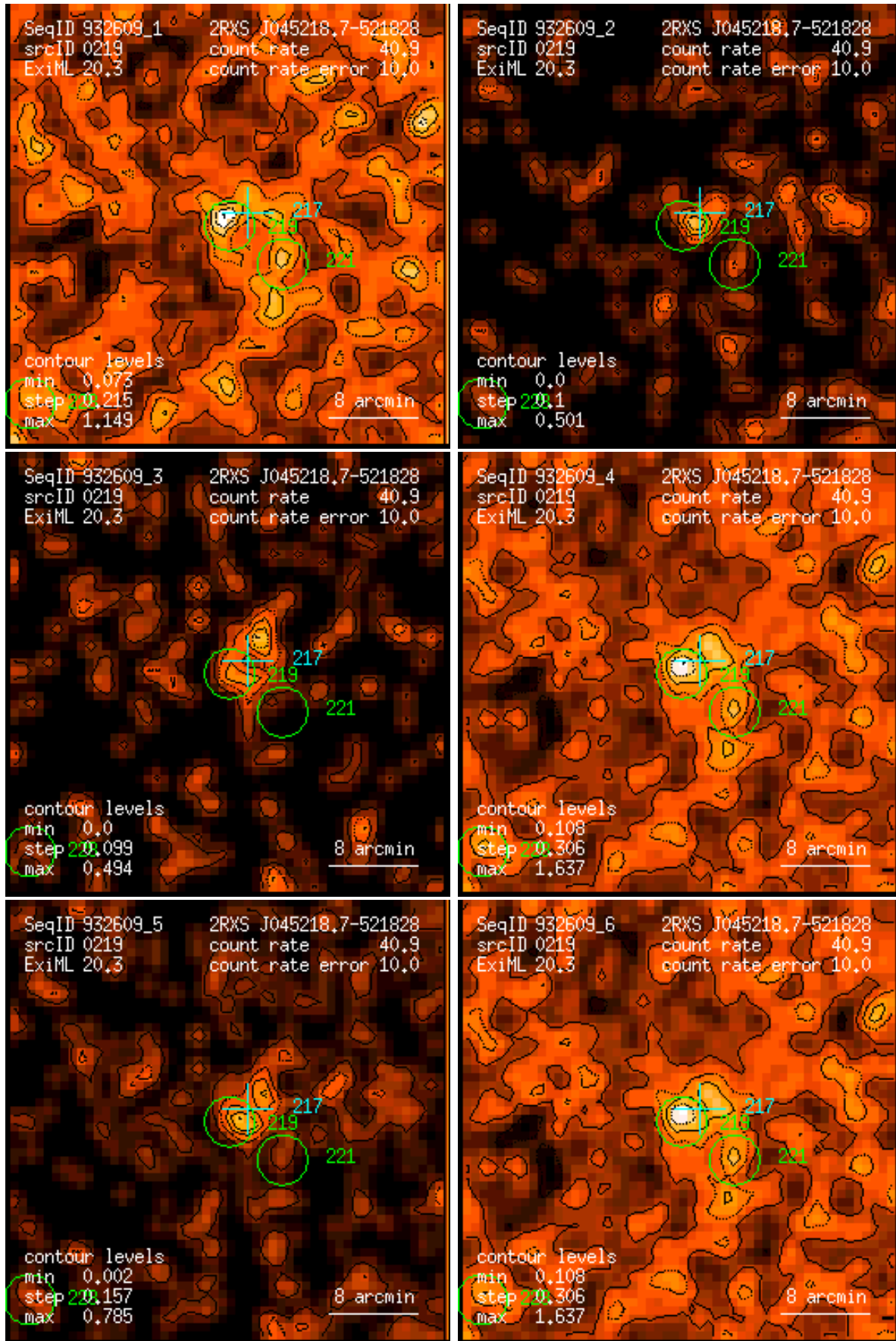
Figure 219: RASS 932609: detection 0219: band rate images, Gaussian filter: (1) PSPC channels 11 – 41, (2) 52 – 90, (3) 91 – 201, (4) 11 – 235, (5) 52 – 201, (6) 11 – 201. Broad band rates in counts/ks. Band rate contour levels in counts/ks/arcmin 2 .
