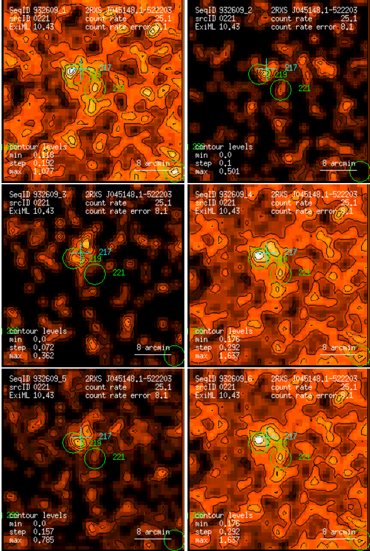
Figure 221: RASS 932609: detection 0221: band rate images, Gaussian filter: (1) PSPC channels 11 – 41, (2) 52 – 90, (3) 91 – 201, (4) 11 – 235, (5) 52 – 201, (6) 11 – 201. Broad band rates in counts/ks. Band rate contour levels in counts/ks/arcmin 2 .
