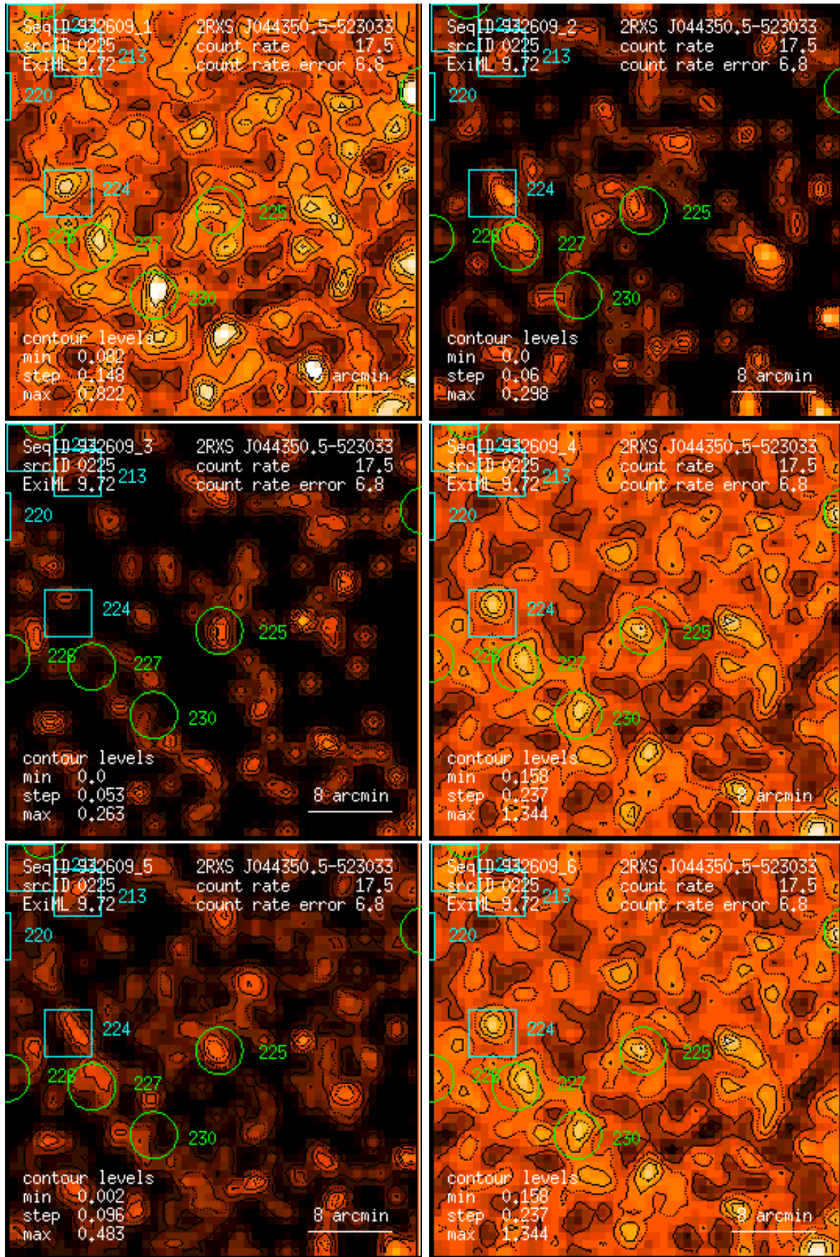
Figure 225: RASS 932609: detection 0225: band rate images, Gaussian filter: (1) PSPC channels 11 – 41, (2) 52 – 90, (3) 91 – 201, (4) 11 – 235, (5) 52 – 201, (6) 11 – 201. Broad band rates in counts/ks. Band rate contour levels in counts/ks/arcmin 2 .
