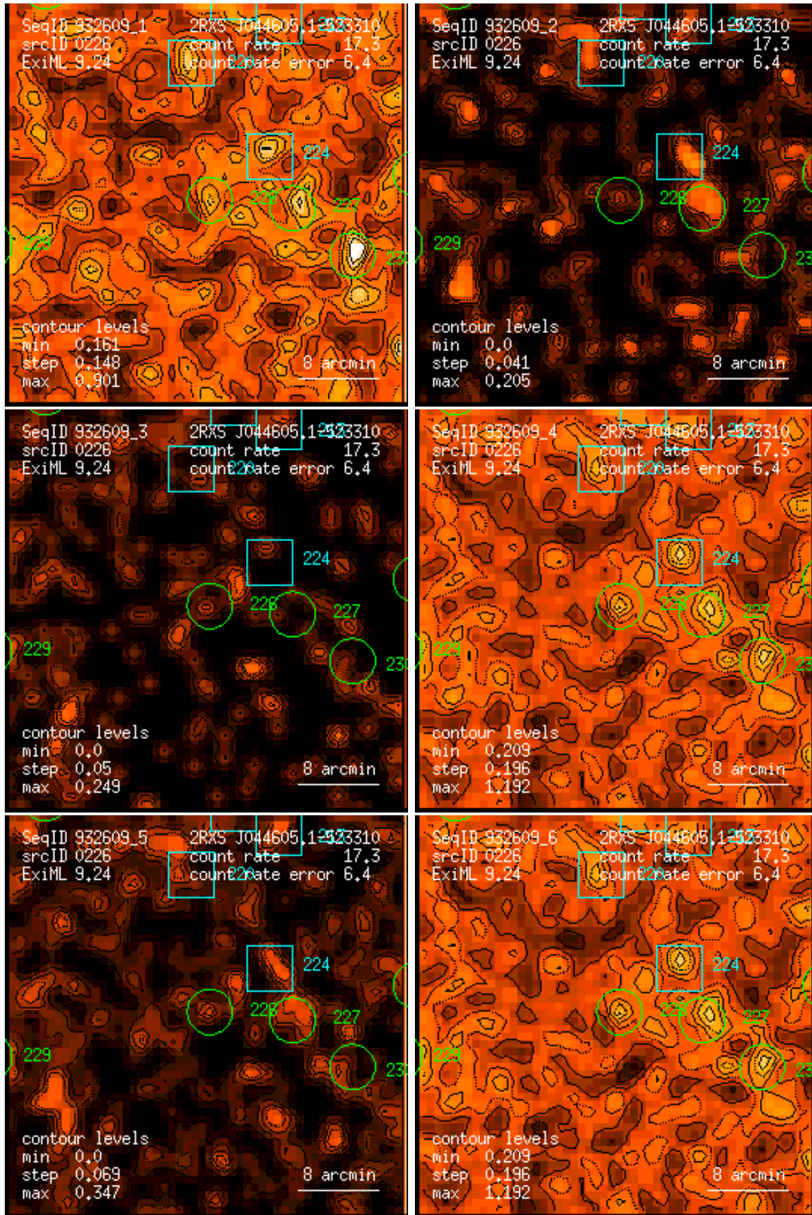
Figure 226: RASS 932609: detection 0226: band rate images, Gaussian filter: (1) PSPC channels 11 – 41, (2) 52 – 90, (3) 91 – 201, (4) 11 – 235, (5) 52 – 201, (6) 11 – 201. Broad band rates in counts/ks. Band rate contour levels in counts/ks/arcmin 2 .
