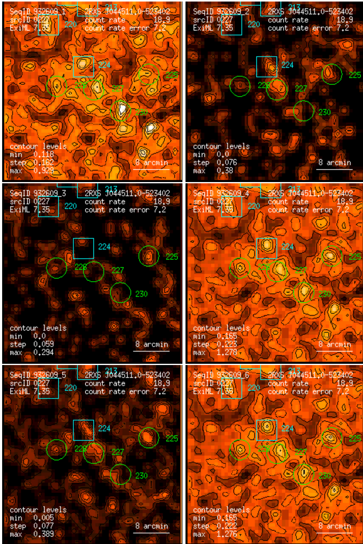
Figure 227: RASS 932609: detection 0227: band rate images, Gaussian filter: (1) PSPC channels 11 – 41, (2) 52 – 90, (3) 91 – 201, (4) 11 – 235, (5) 52 – 201, (6) 11 – 201. Broad band rates in counts/ks. Band rate contour levels in counts/ks/arcmin 2 .
