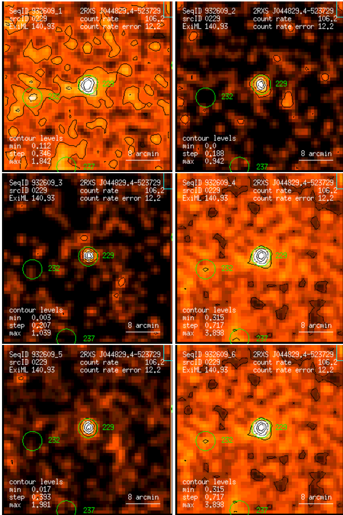
Figure 229: RASS 932609: detection 0229: band rate images, Gaussian filter: (1) PSPC channels 11 – 41, (2) 52 – 90, (3) 91 – 201, (4) 11 – 235, (5) 52 – 201, (6) 11 – 201. Broad band rates in counts/ks. Band rate contour levels in counts/ks/arcmin 2 .
