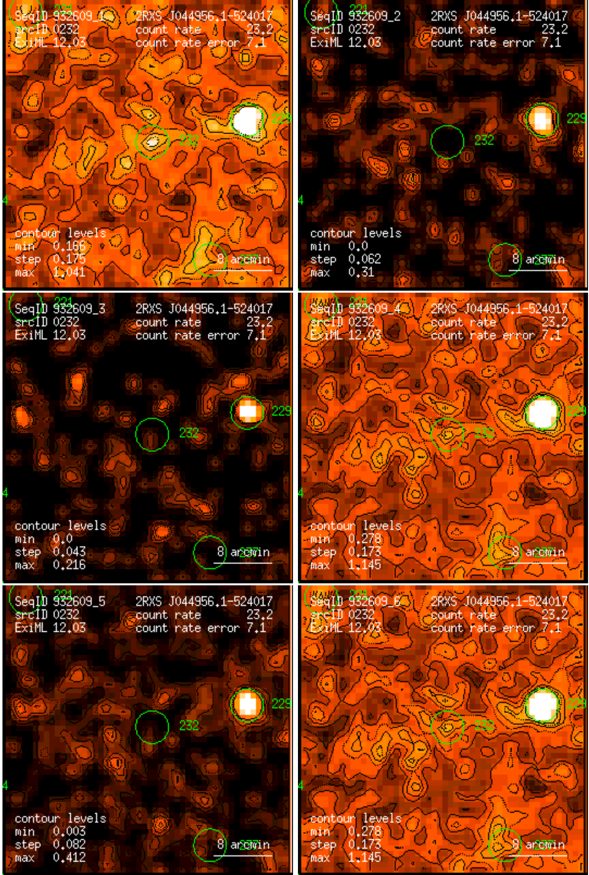
Figure 232: RASS 932609: detection 0232: band rate images, Gaussian filter: (1) PSPC channels 11 – 41, (2) 52 – 90, (3) 91 – 201, (4) 11 – 235, (5) 52 – 201, (6) 11 – 201. Broad band rates in counts/ks. Band rate contour levels in counts/ks/arcmin 2 .
