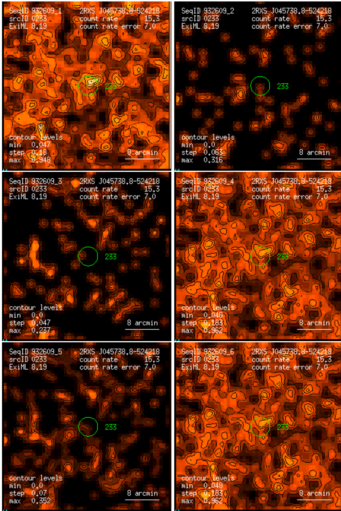
Figure 233: RASS 932609: detection 0233: band rate images, Gaussian filter: (1) PSPC channels 11 – 41, (2) 52 – 90, (3) 91 – 201, (4) 11 – 235, (5) 52 – 201, (6) 11 – 201. Broad band rates in counts/ks. Band rate contour levels in counts/ks/arcmin 2 .
