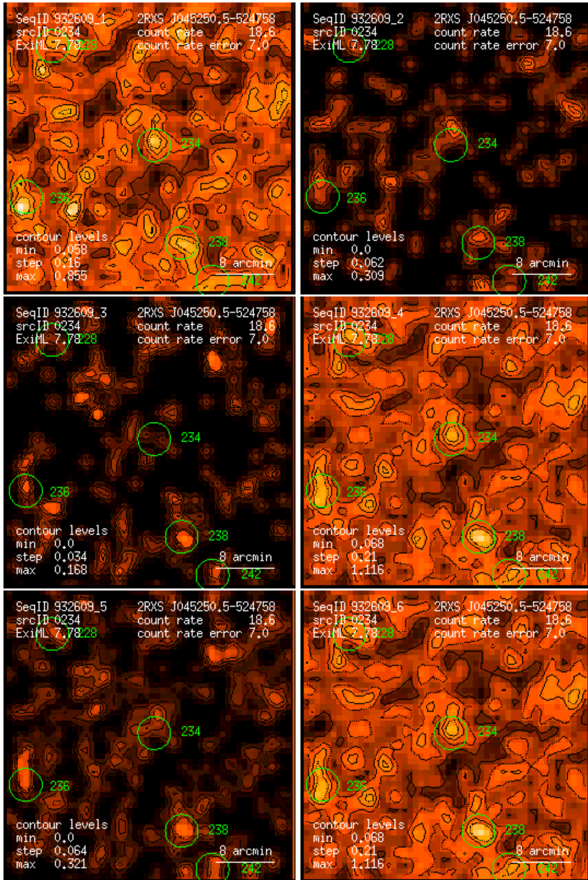
Figure 234: RASS 932609: detection 0234: band rate images, Gaussian filter: (1) PSPC channels 11 – 41, (2) 52 – 90, (3) 91 – 201, (4) 11 – 235, (5) 52 – 201, (6) 11 – 201. Broad band rates in counts/ks. Band rate contour levels in counts/ks/arcmin 2 .
