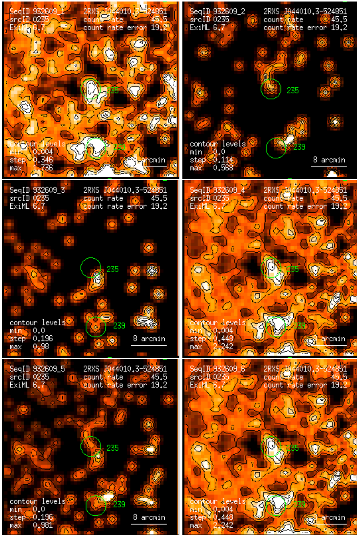
Figure 235: RASS 932609: detection 0235: band rate images, Gaussian filter: (1) PSPC channels 11 – 41, (2) 52 – 90, (3) 91 – 201, (4) 11 – 235, (5) 52 – 201, (6) 11 – 201. Broad band rates in counts/ks. Band rate contour levels in counts/ks/arcmin 2 .
