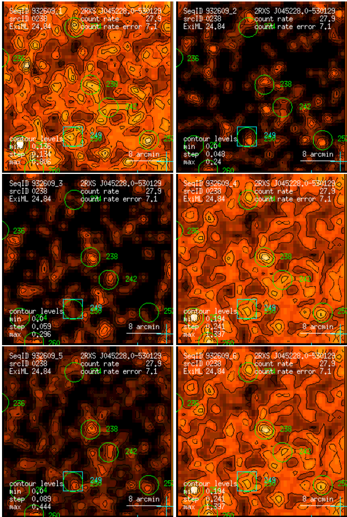
Figure 238: RASS 932609: detection 0238: band rate images, Gaussian filter: (1) PSPC channels 11 – 41, (2) 52 – 90, (3) 91 – 201, (4) 11 – 235, (5) 52 – 201, (6) 11 – 201. Broad band rates in counts/ks. Band rate contour levels in counts/ks/arcmin 2 .
