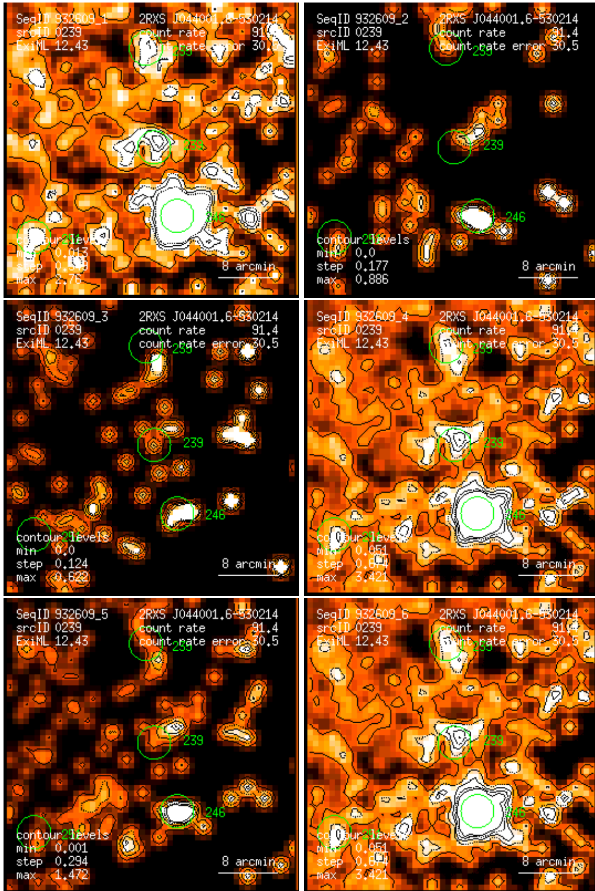
Figure 239: RASS 932609: detection 0239: band rate images, Gaussian filter: (1) PSPC channels 11 – 41, (2) 52 – 90, (3) 91 – 201, (4) 11 – 235, (5) 52 – 201, (6) 11 – 201. Broad band rates in counts/ks. Band rate contour levels in counts/ks/arcmin 2 .
