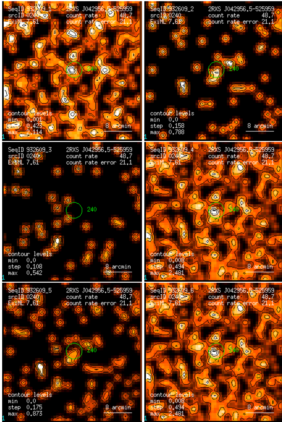
Figure 240: RASS 932609: detection 0240: band rate images, Gaussian filter: (1) PSPC channels 11 – 41, (2) 52 – 90, (3) 91 – 201, (4) 11 – 235, (5) 52 – 201, (6) 11 – 201. Broad band rates in counts/ks. Band rate contour levels in counts/ks/arcmin 2 .
