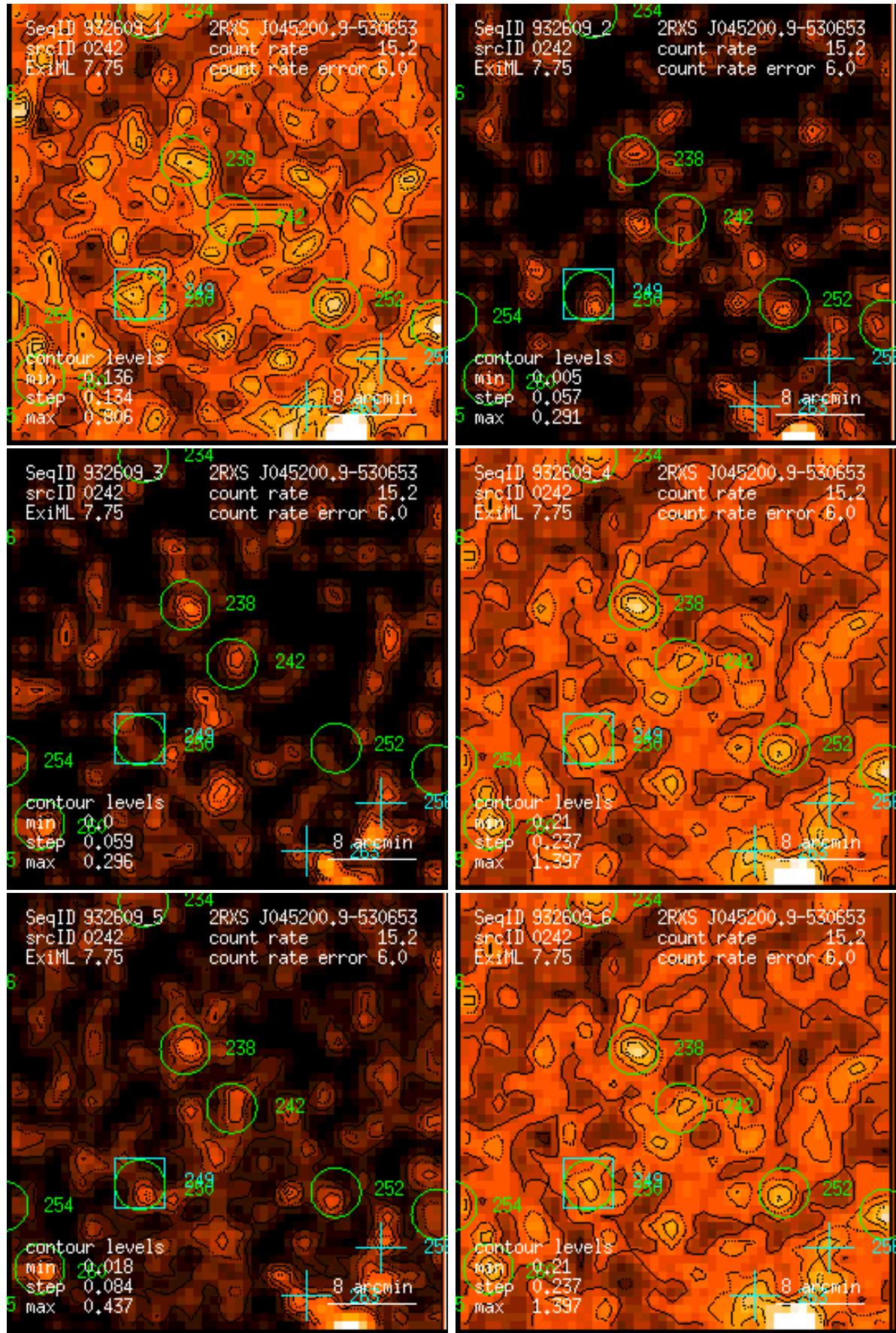
Figure 242: RASS 932609: detection 0242: band rate images, Gaussian filter: (1) PSPC channels 11 – 41, (2) 52 – 90, (3) 91 – 201, (4) 11 – 235, (5) 52 – 201, (6) 11 – 201. Broad band rates in counts/ks. Band rate contour levels in counts/ks/arcmin 2 .
