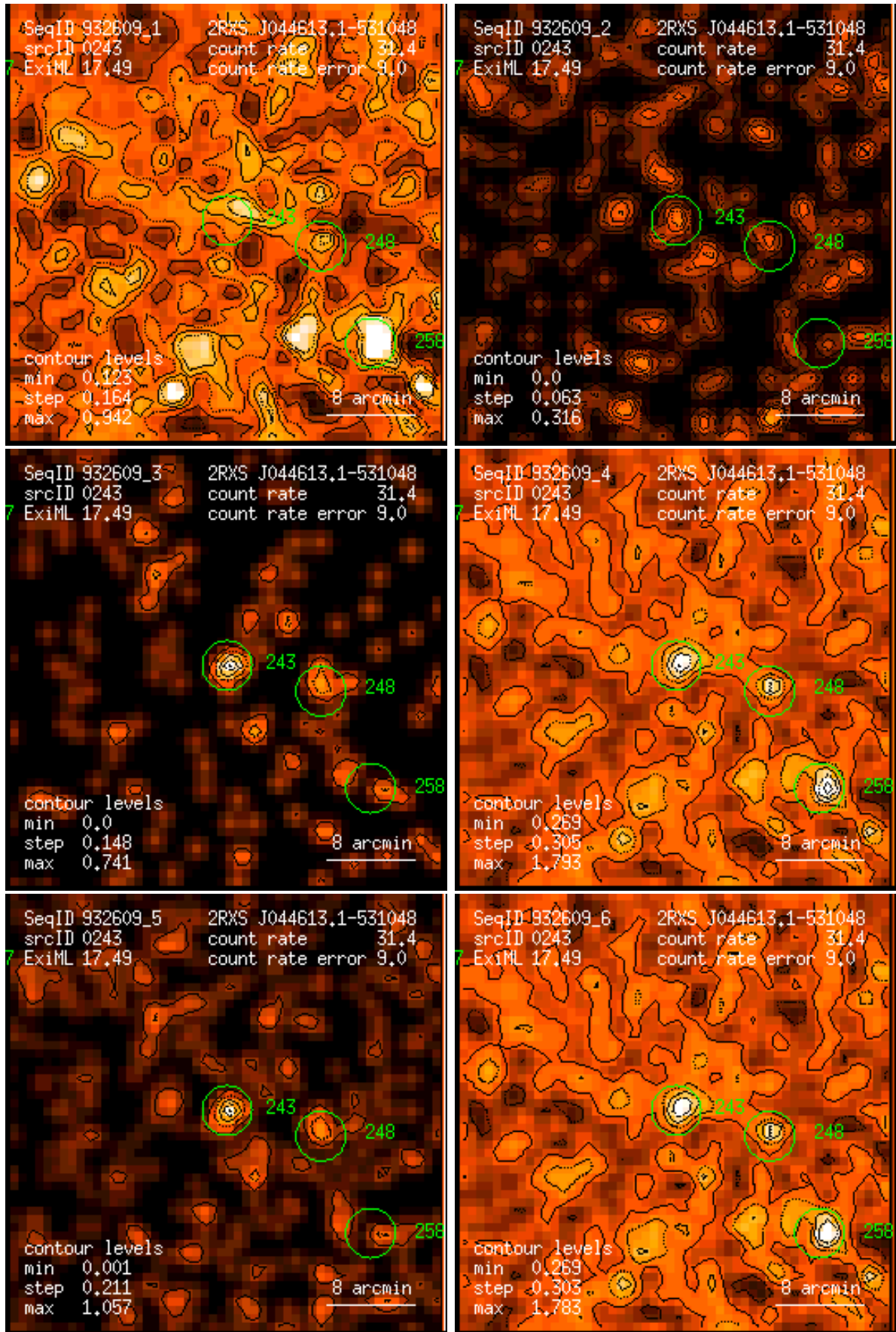
Figure 243: RASS 932609: detection 0243: band rate images, Gaussian filter: (1) PSPC channels 11 – 41, (2) 52 – 90, (3) 91 – 201, (4) 11 – 235, (5) 52 – 201, (6) 11 – 201. Broad band rates in counts/ks. Band rate contour levels in counts/ks/arcmin 2 .
