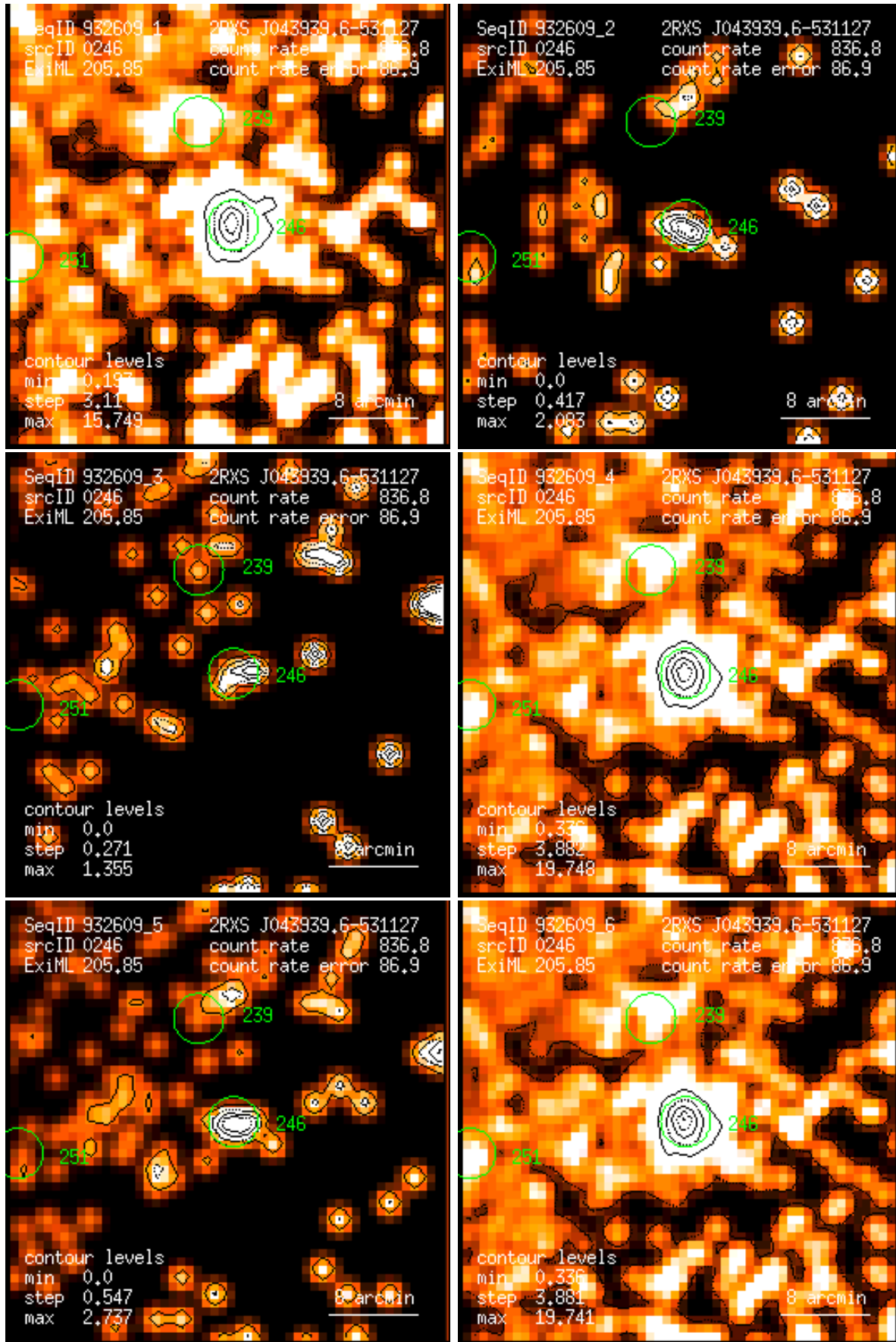
Figure 246: RASS 932609: detection 0246: band rate images, Gaussian filter: (1) PSPC channels 11 – 41, (2) 52 – 90, (3) 91 – 201, (4) 11 – 235, (5) 52 – 201, (6) 11 – 201. Broad band rates in counts/ks. Band rate contour levels in counts/ks/arcmin 2 .
