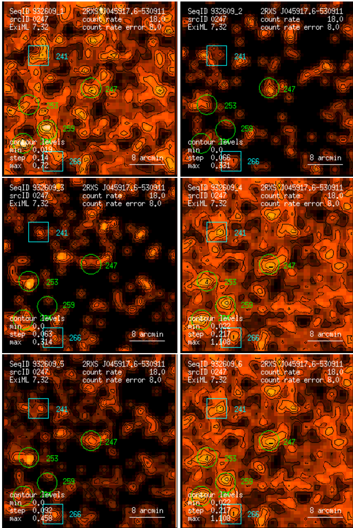
Figure 247: RASS 932609: detection 0247: band rate images, Gaussian filter: (1) PSPC channels 11 – 41, (2) 52 – 90, (3) 91 – 201, (4) 11 – 235, (5) 52 – 201, (6) 11 – 201. Broad band rates in counts/ks. Band rate contour levels in counts/ks/arcmin 2 .
