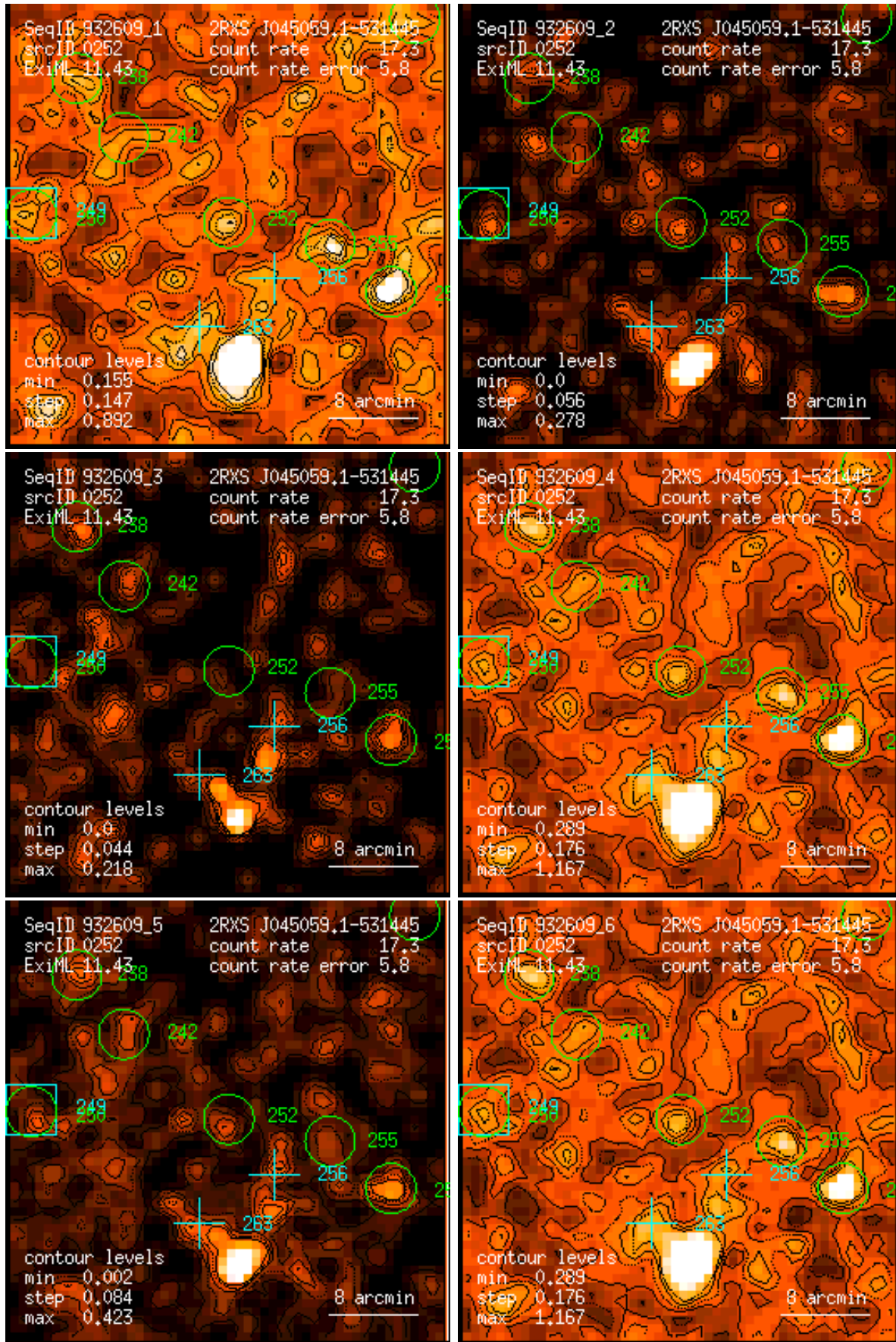
Figure 252: RASS 932609: detection 0252: band rate images, Gaussian filter: (1) PSPC channels 11 – 41, (2) 52 – 90, (3) 91 – 201, (4) 11 – 235, (5) 52 – 201, (6) 11 – 201. Broad band rates in counts/ks. Band rate contour levels in counts/ks/arcmin 2 .
