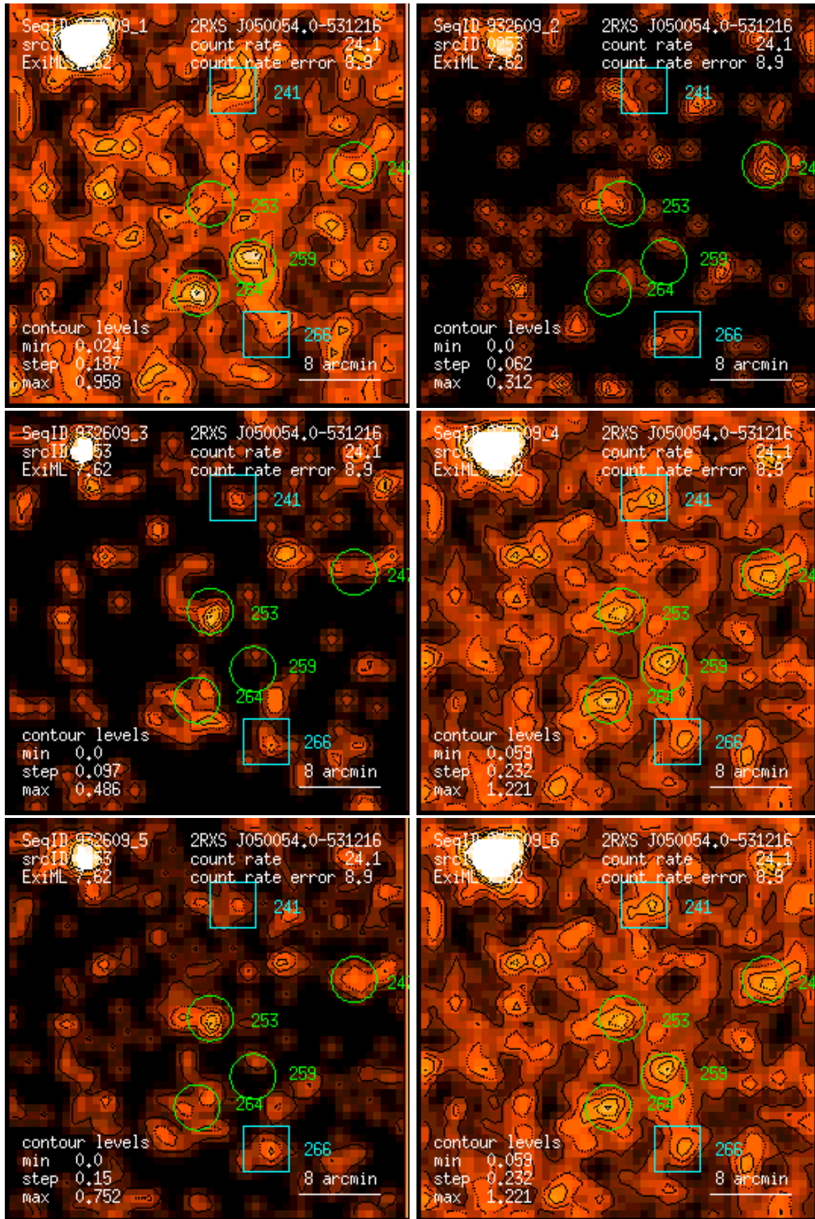
Figure 253: RASS 932609: detection 0253: band rate images, Gaussian filter: (1) PSPC channels 11 – 41, (2) 52 – 90, (3) 91 – 201, (4) 11 – 235, (5) 52 – 201, (6) 11 – 201. Broad band rates in counts/ks. Band rate contour levels in counts/ks/arcmin 2 .
