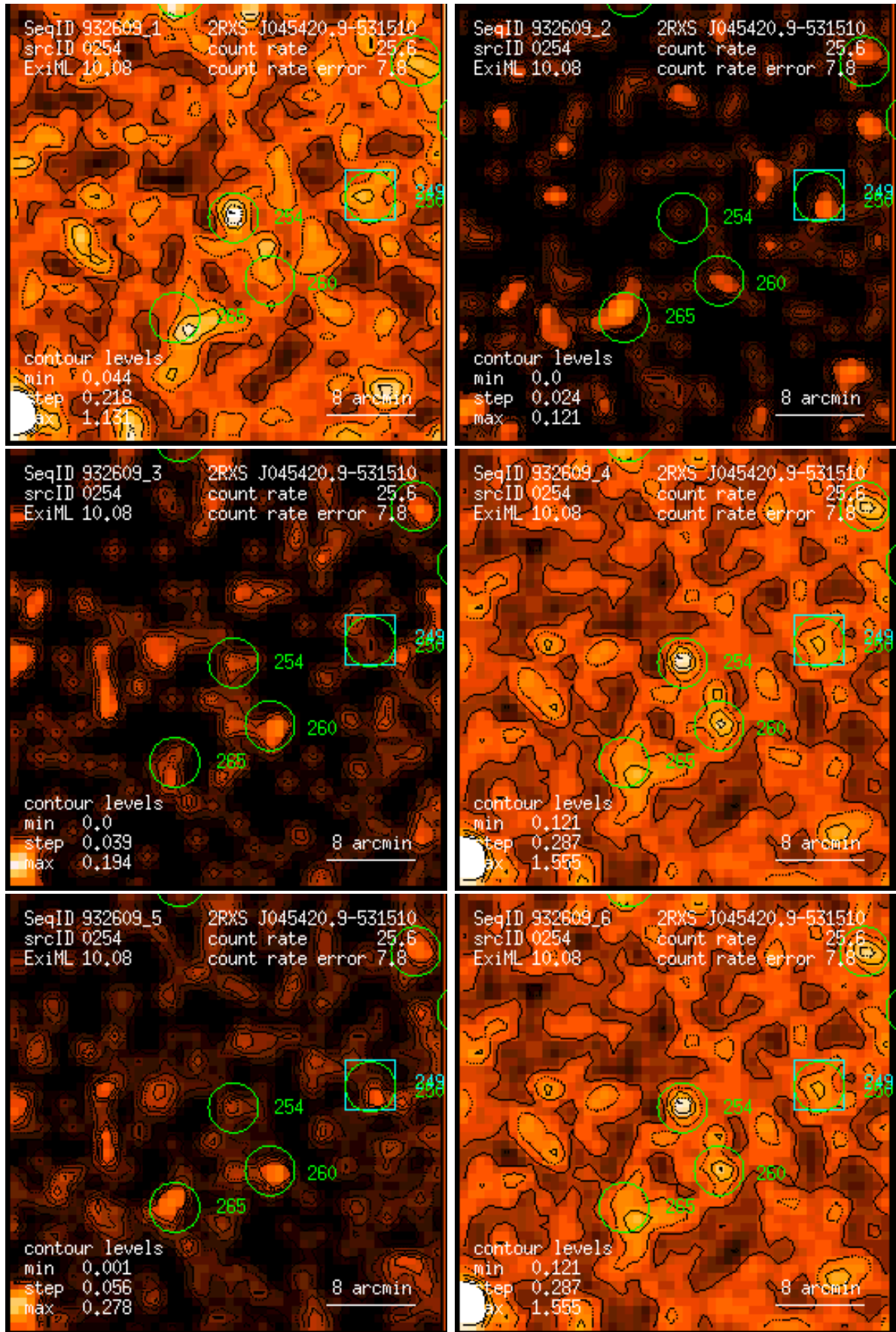
Figure 254: RASS 932609: detection 0254: band rate images, Gaussian filter: (1) PSPC channels 11 – 41, (2) 52 – 90, (3) 91 – 201, (4) 11 – 235, (5) 52 – 201, (6) 11 – 201. Broad band rates in counts/ks. Band rate contour levels in counts/ks/arcmin 2 .
