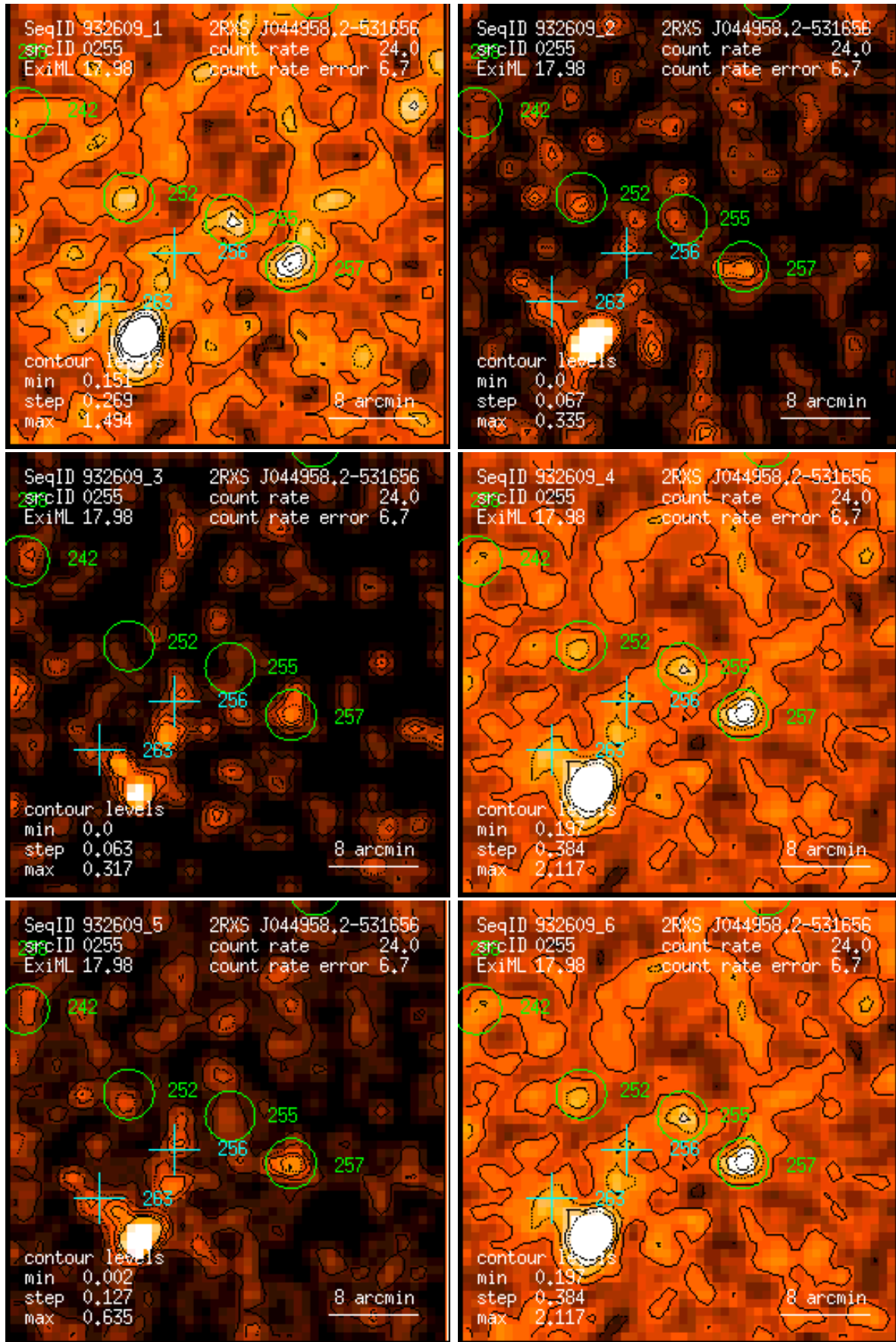
Figure 255: RASS 932609: detection 0255: band rate images, Gaussian filter: (1) PSPC channels 11 – 41, (2) 52 – 90, (3) 91 – 201, (4) 11 – 235, (5) 52 – 201, (6) 11 – 201. Broad band rates in counts/ks. Band rate contour levels in counts/ks/arcmin 2 .
