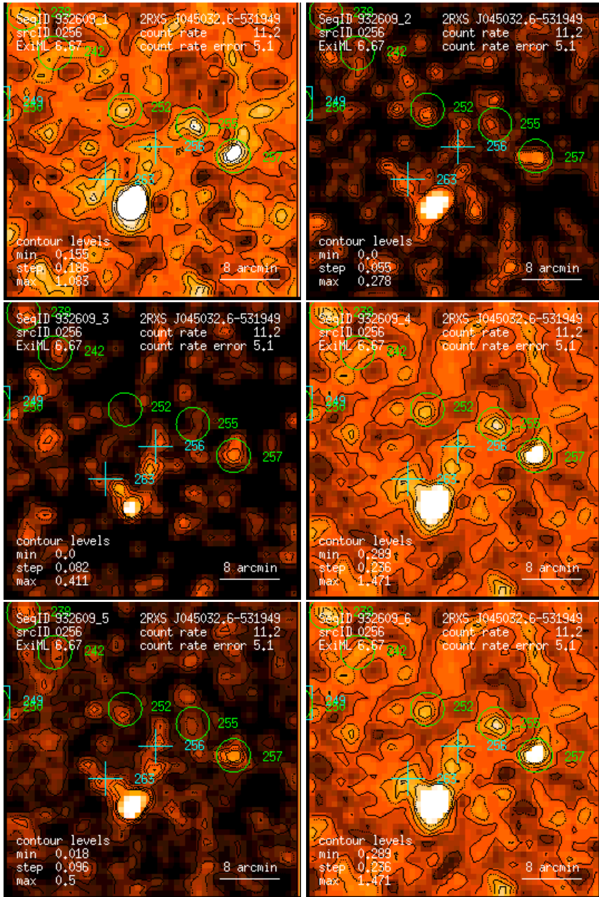
Figure 256: RASS 932609: detection 0256: band rate images, Gaussian filter: (1) PSPC channels 11 – 41, (2) 52 – 90, (3) 91 – 201, (4) 11 – 235, (5) 52 – 201, (6) 11 – 201. Broad band rates in counts/ks. Band rate contour levels in counts/ks/arcmin 2 .
