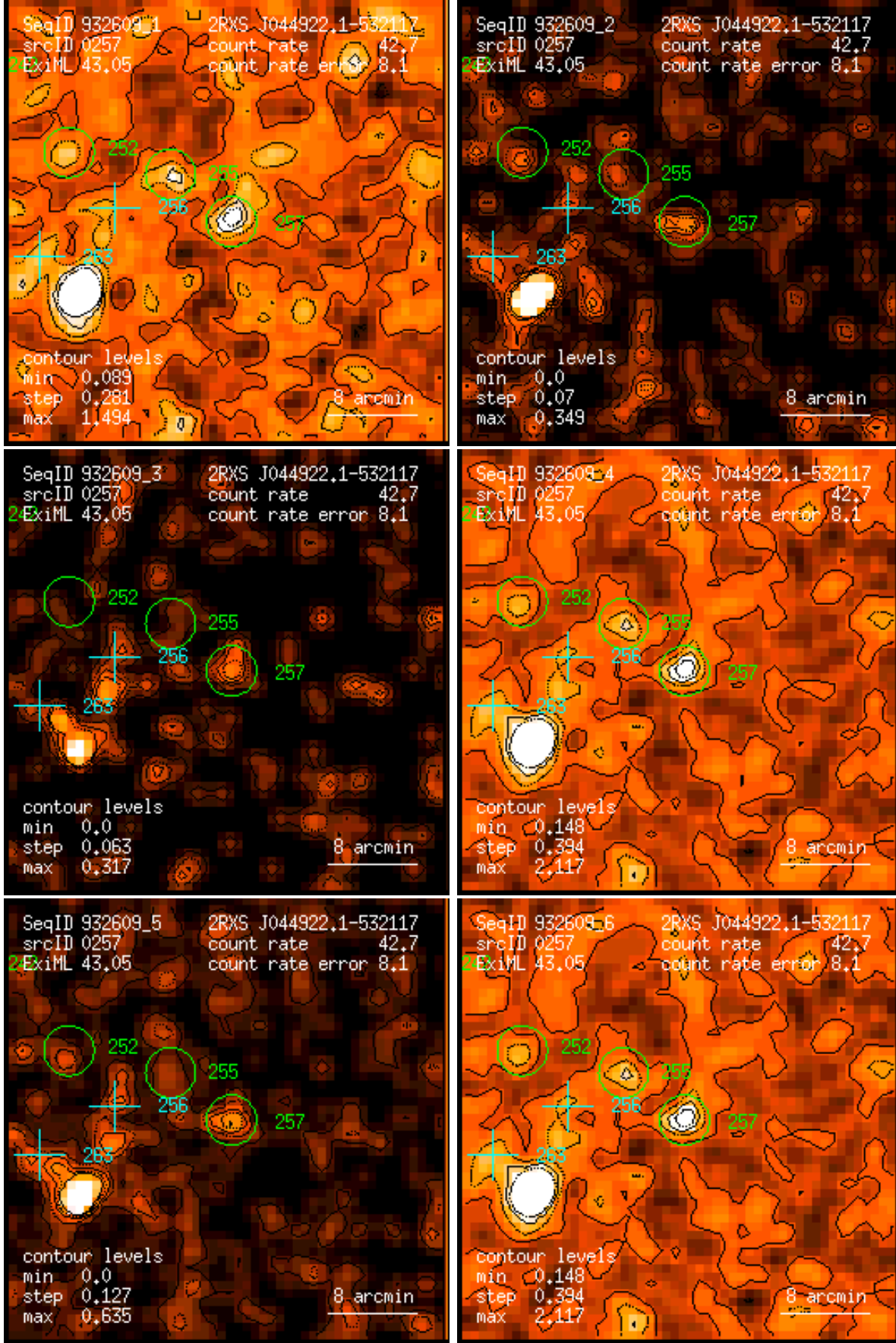
Figure 257: RASS 932609: detection 0257: band rate images, Gaussian filter: (1) PSPC channels 11 – 41, (2) 52 – 90, (3) 91 – 201, (4) 11 – 235, (5) 52 – 201, (6) 11 – 201. Broad band rates in counts/ks. Band rate contour levels in counts/ks/arcmin 2 .
