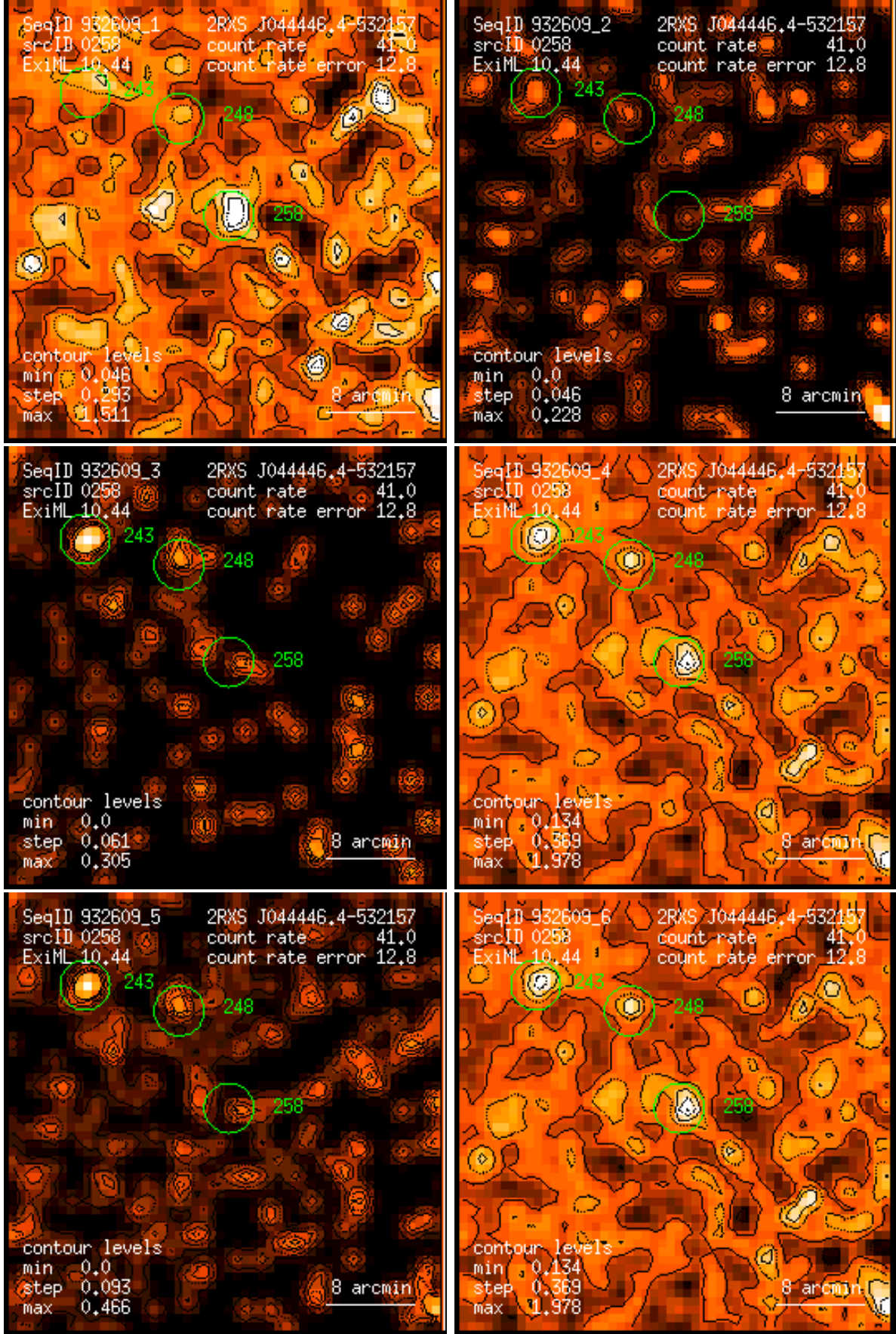
Figure 258: RASS 932609: detection 0258: band rate images, Gaussian filter: (1) PSPC channels 11 – 41, (2) 52 – 90, (3) 91 – 201, (4) 11 – 235, (5) 52 – 201, (6) 11 – 201. Broad band rates in counts/ks. Band rate contour levels in counts/ks/arcmin 2 .
