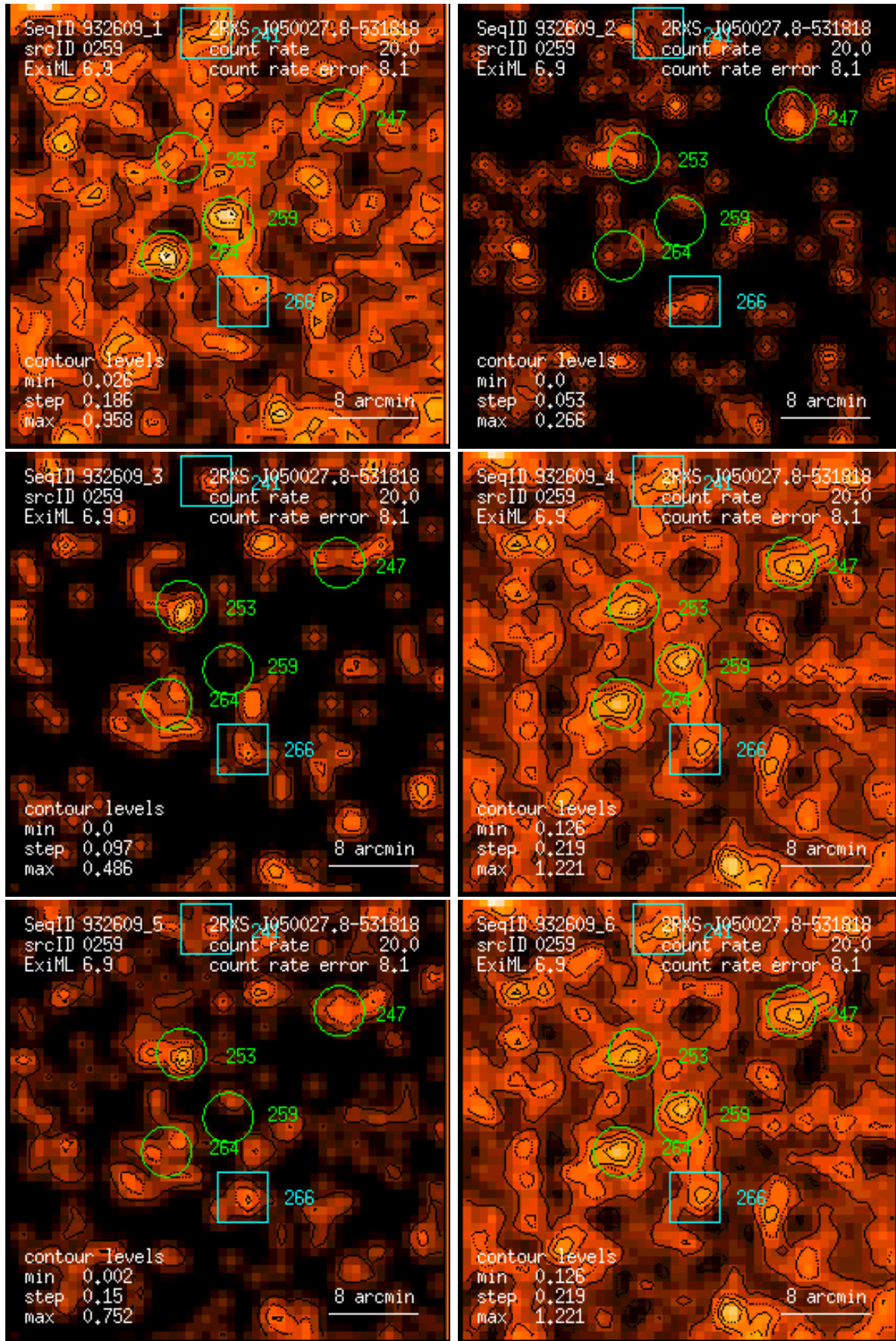
Figure 259: RASS 932609: detection 0259: band rate images, Gaussian filter: (1) PSPC channels 11 – 41, (2) 52 – 90, (3) 91 – 201, (4) 11 – 235, (5) 52 – 201, (6) 11 – 201. Broad band rates in counts/ks. Band rate contour levels in counts/ks/arcmin 2 .
