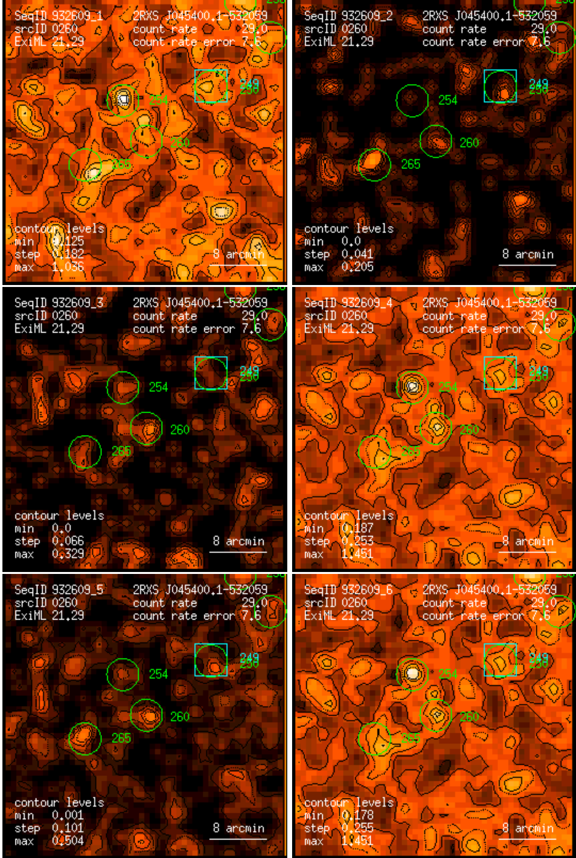
Figure 260: RASS 932609: detection 0260: band rate images, Gaussian filter: (1) PSPC channels 11 – 41, (2) 52 – 90, (3) 91 – 201, (4) 11 – 235, (5) 52 – 201, (6) 11 – 201. Broad band rates in counts/ks. Band rate contour levels in counts/ks/arcmin 2 .
