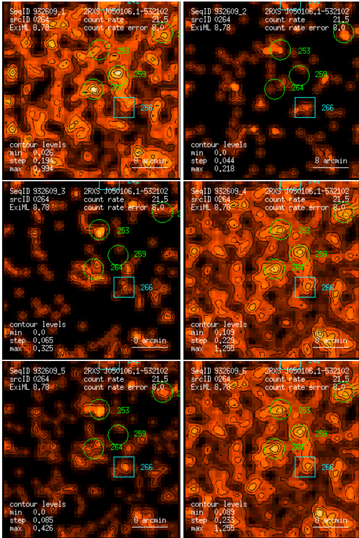
Figure 264: RASS 932609: detection 0264: band rate images, Gaussian filter: (1) PSPC channels 11 – 41, (2) 52 – 90, (3) 91 – 201, (4) 11 – 235, (5) 52 – 201, (6) 11 – 201. Broad band rates in counts/ks. Band rate contour levels in counts/ks/arcmin 2 .
