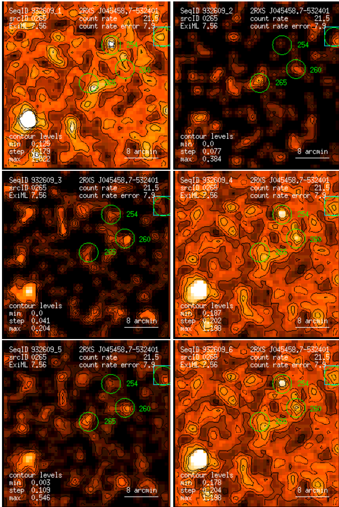
Figure 265: RASS 932609: detection 0265: band rate images, Gaussian filter: (1) PSPC channels 11 – 41, (2) 52 – 90, (3) 91 – 201, (4) 11 – 235, (5) 52 – 201, (6) 11 – 201. Broad band rates in counts/ks. Band rate contour levels in counts/ks/arcmin 2 .
