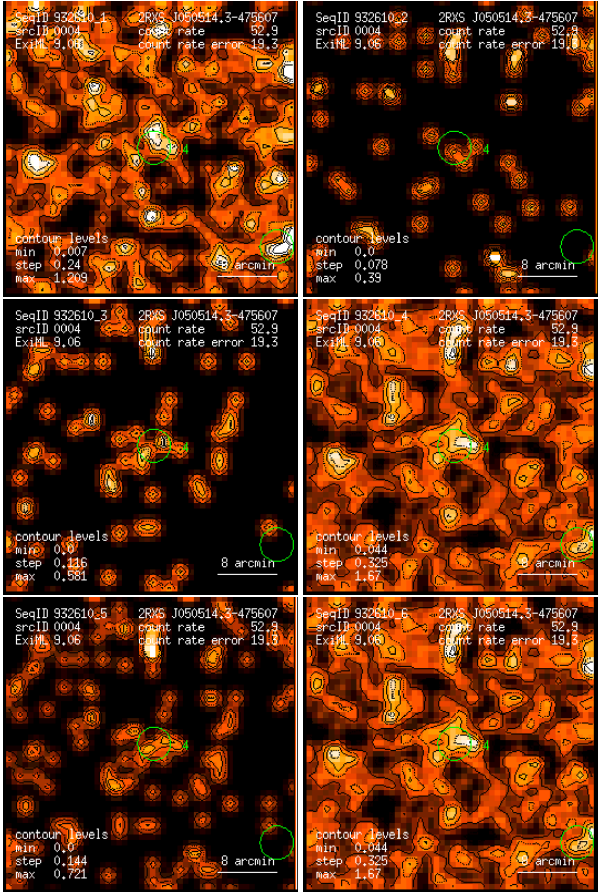
Figure 4: RASS 932610: detection 0004: band rate images, Gaussian filter: (1) PSPC channels 11 – 41, (2) 52 – 90, (3) 91 – 201, (4) 11 – 235, (5) 52 – 201, (6) 11 – 201. Broad band rates in counts/ks. Band rate contour levels in counts/ks/arcmin 2 .
