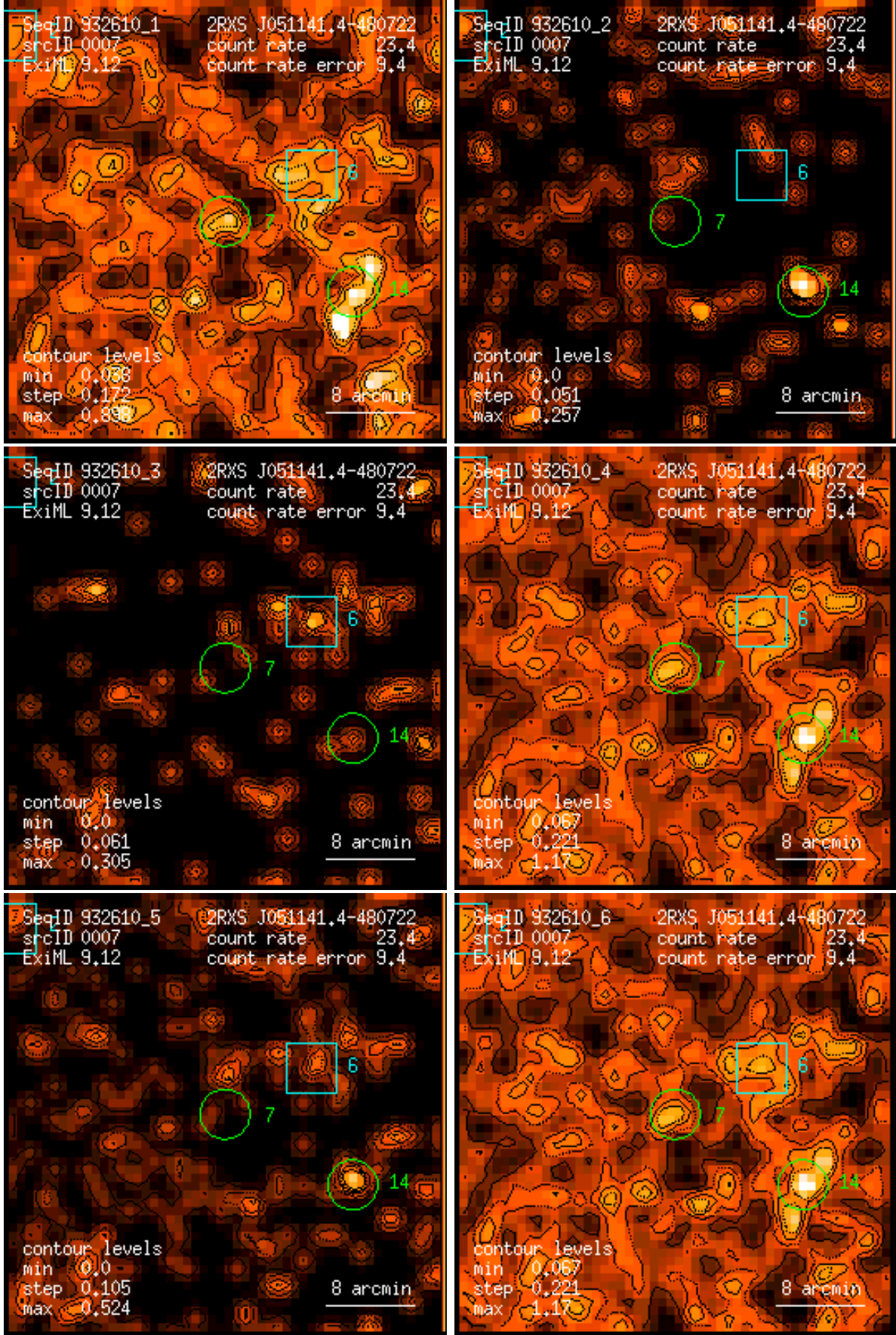
Figure 7: RASS 932610: detection 0007: band rate images, Gaussian filter: (1) PSPC channels 11 – 41, (2) 52 – 90, (3) 91 – 201, (4) 11 – 235, (5) 52 – 201, (6) 11 – 201. Broad band rates in counts/ks. Band rate contour levels in counts/ks/arcmin 2 .
