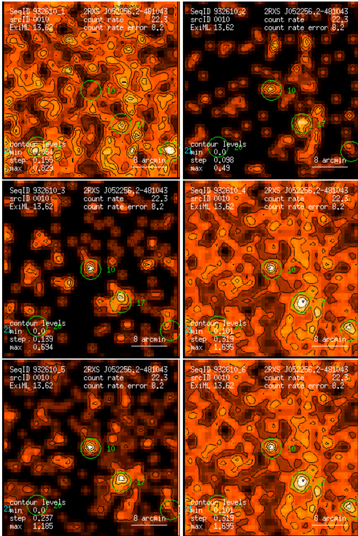
Figure 10: RASS 932610: detection 0010: band rate images, Gaussian filter: (1) PSPC channels 11 – 41, (2) 52 – 90, (3) 91 – 201, (4) 11 – 235, (5) 52 – 201, (6) 11 – 201. Broad band rates in counts/ks. Band rate contour levels in counts/ks/arcmin 2 .
