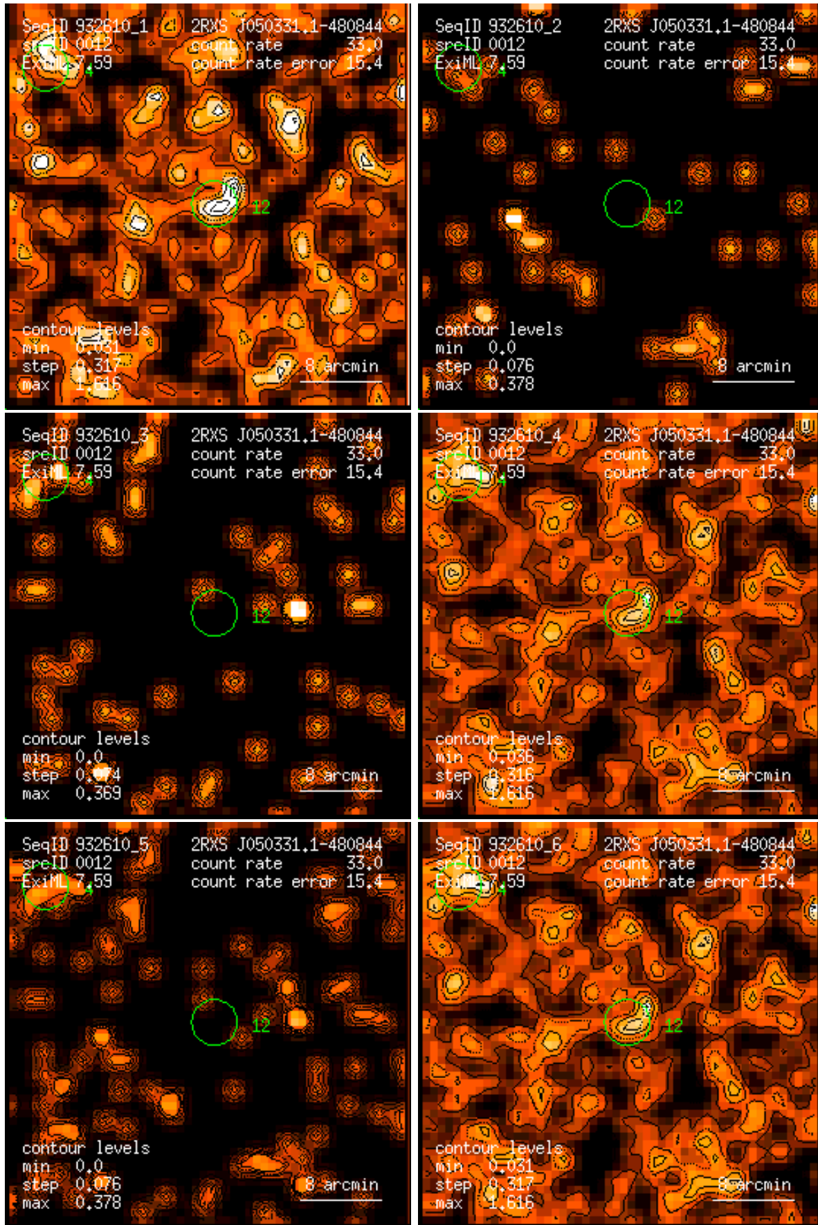
Figure 12: RASS 932610: detection 0012: band rate images, Gaussian filter: (1) PSPC channels 11 – 41, (2) 52 – 90, (3) 91 – 201, (4) 11 – 235, (5) 52 – 201, (6) 11 – 201. Broad band rates in counts/ks. Band rate contour levels in counts/ks/arcmin 2 .
