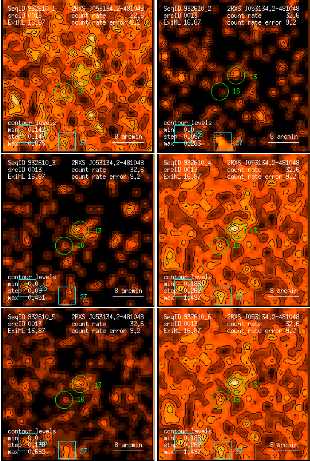
Figure 13: RASS 932610: detection 0013: band rate images, Gaussian filter: (1) PSPC channels 11 – 41, (2) 52 – 90, (3) 91 – 201, (4) 11 – 235, (5) 52 – 201, (6) 11 – 201. Broad band rates in counts/ks. Band rate contour levels in counts/ks/arcmin 2 .
