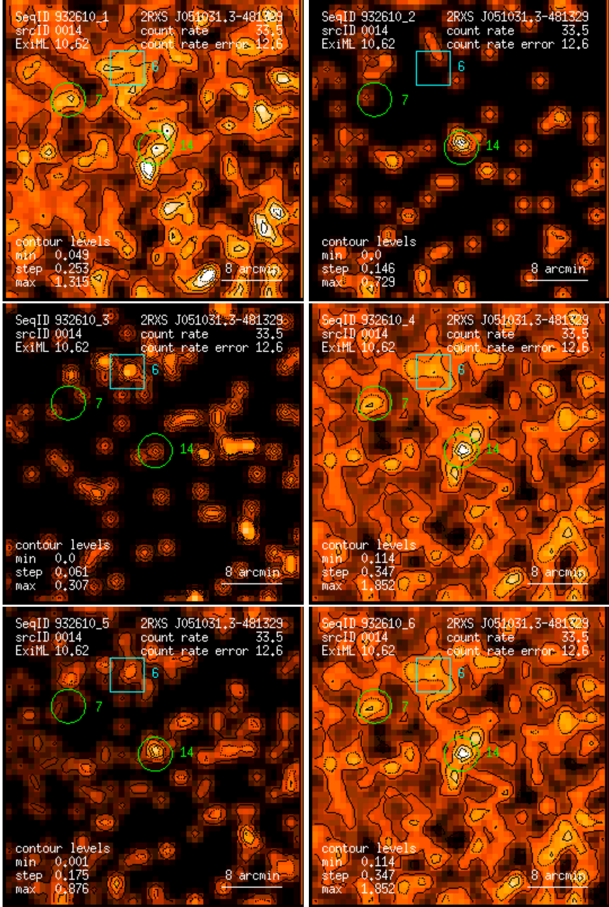
Figure 14: RASS 932610: detection 0014: band rate images, Gaussian filter: (1) PSPC channels 11 – 41, (2) 52 – 90, (3) 91 – 201, (4) 11 – 235, (5) 52 – 201, (6) 11 – 201. Broad band rates in counts/ks. Band rate contour levels in counts/ks/arcmin 2 .
