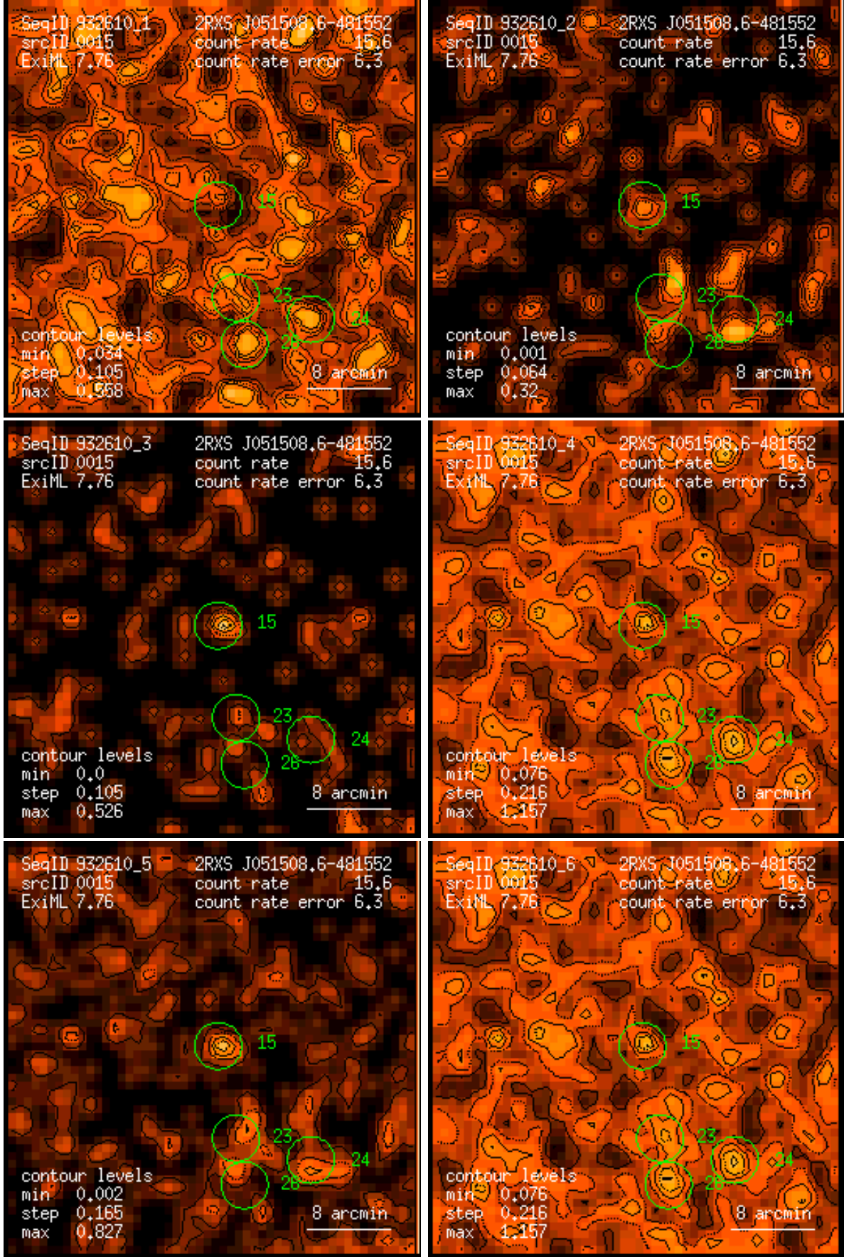
Figure 15: RASS 932610: detection 0015: band rate images, Gaussian filter: (1) PSPC channels 11 – 41, (2) 52 – 90, (3) 91 – 201, (4) 11 – 235, (5) 52 – 201, (6) 11 – 201. Broad band rates in counts/ks. Band rate contour levels in counts/ks/arcmin 2 .
