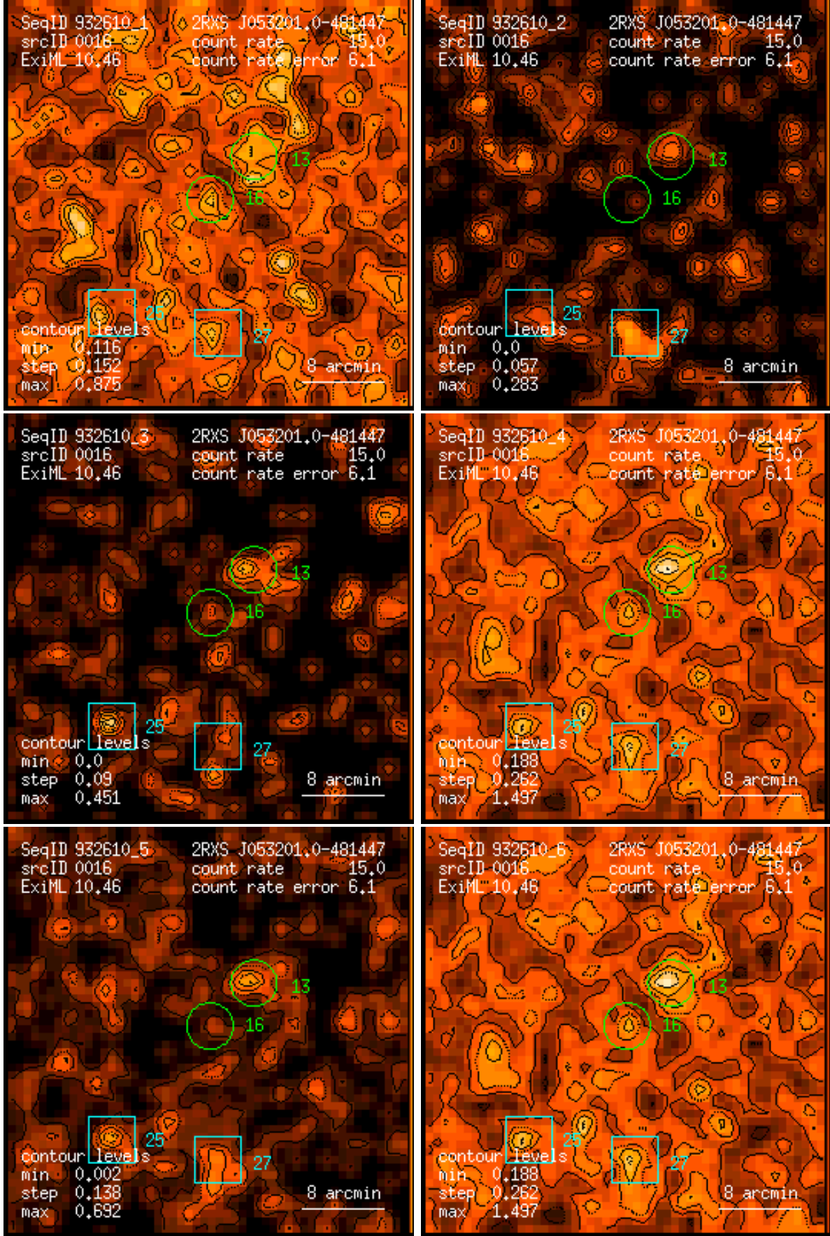
Figure 16: RASS 932610: detection 0016: band rate images, Gaussian filter: (1) PSPC channels 11 – 41, (2) 52 – 90, (3) 91 – 201, (4) 11 – 235, (5) 52 – 201, (6) 11 – 201. Broad band rates in counts/ks. Band rate contour levels in counts/ks/arcmin 2 .
