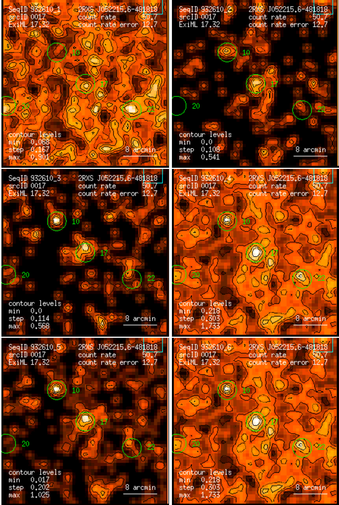
Figure 17: RASS 932610: detection 0017: band rate images, Gaussian filter: (1) PSPC channels 11 – 41, (2) 52 – 90, (3) 91 – 201, (4) 11 – 235, (5) 52 – 201, (6) 11 – 201. Broad band rates in counts/ks. Band rate contour levels in counts/ks/arcmin 2 .
